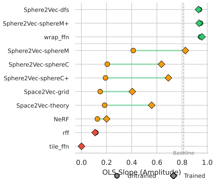
Global \beta_2 : OLS Slope (Amplitude)
