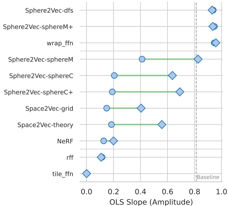
Global \beta_2 : OLS Slope (Amplitude)
