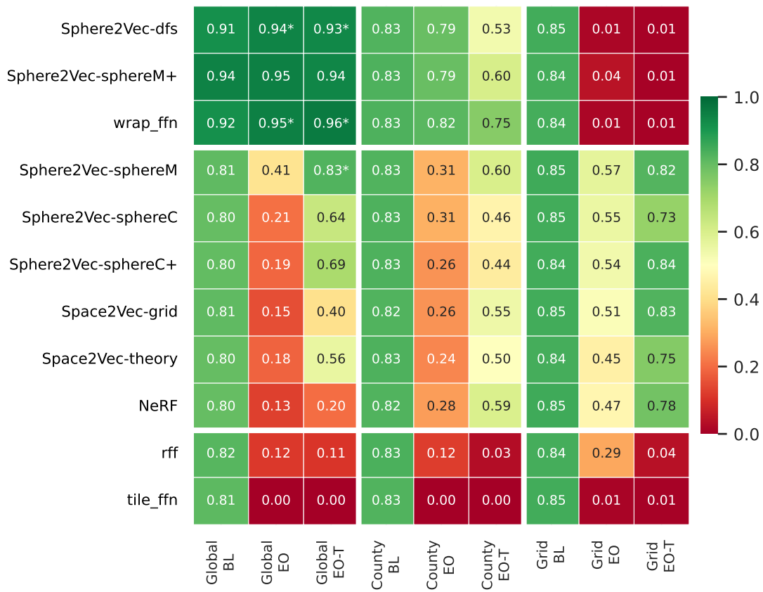
Amplitude Recovery (OLS Slope)
