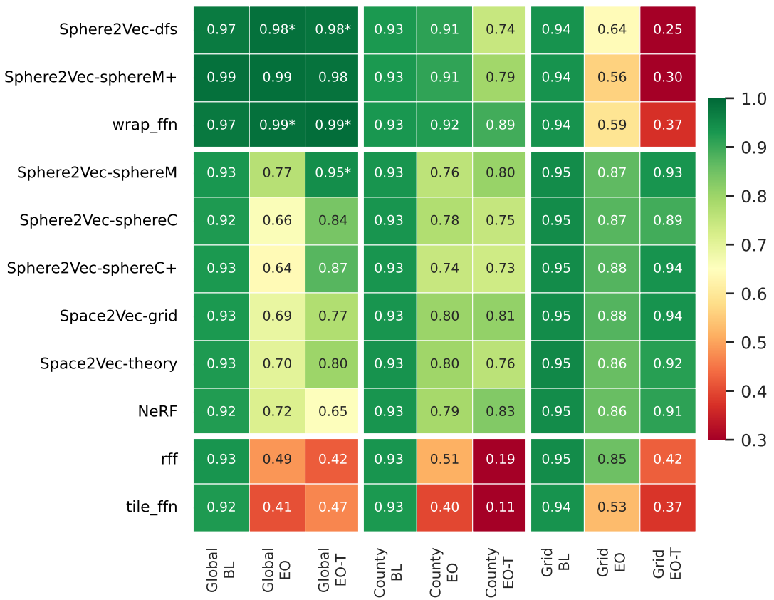
Pattern Recovery (Pearson r )
