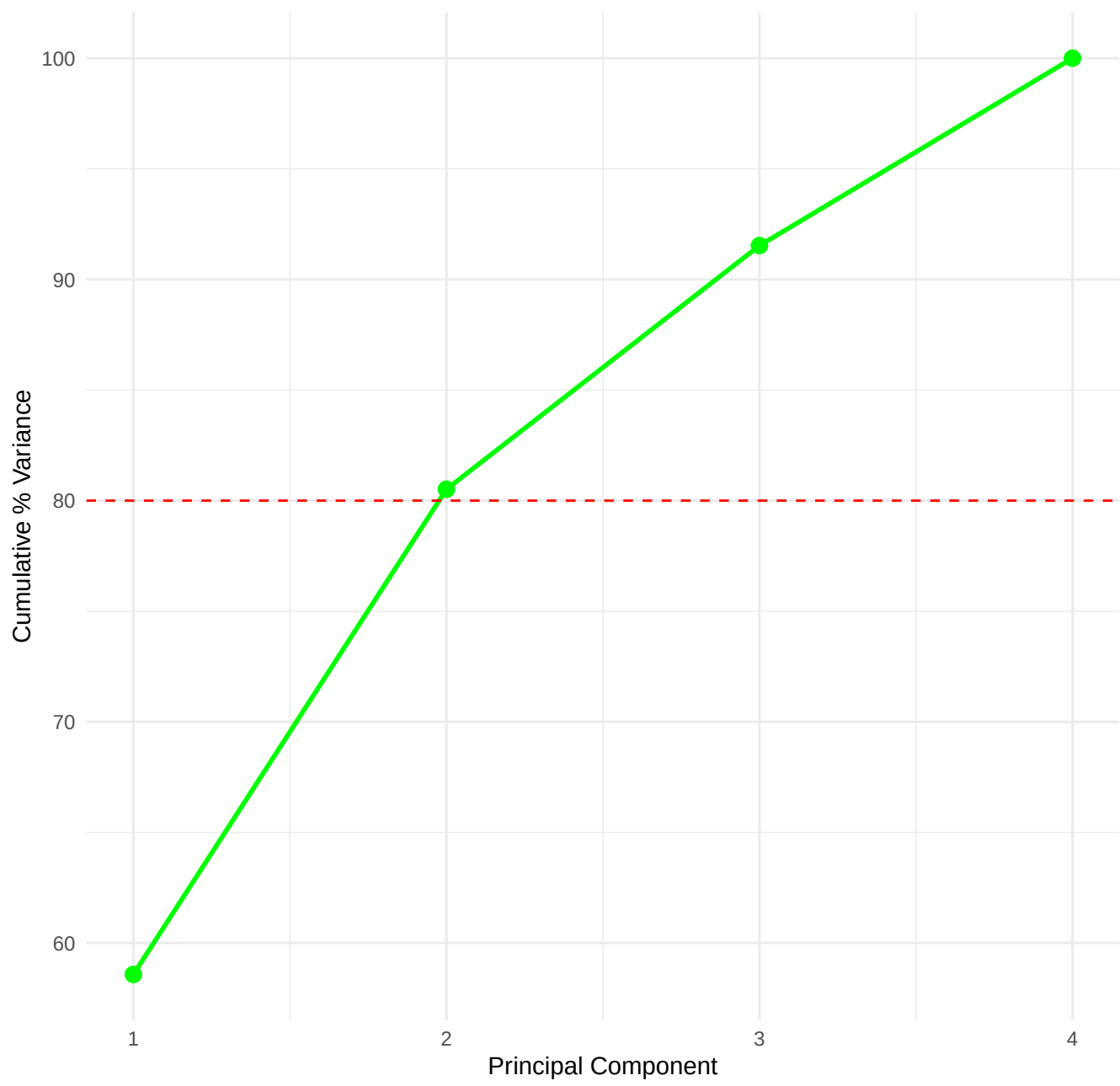
Cumulative Variance
