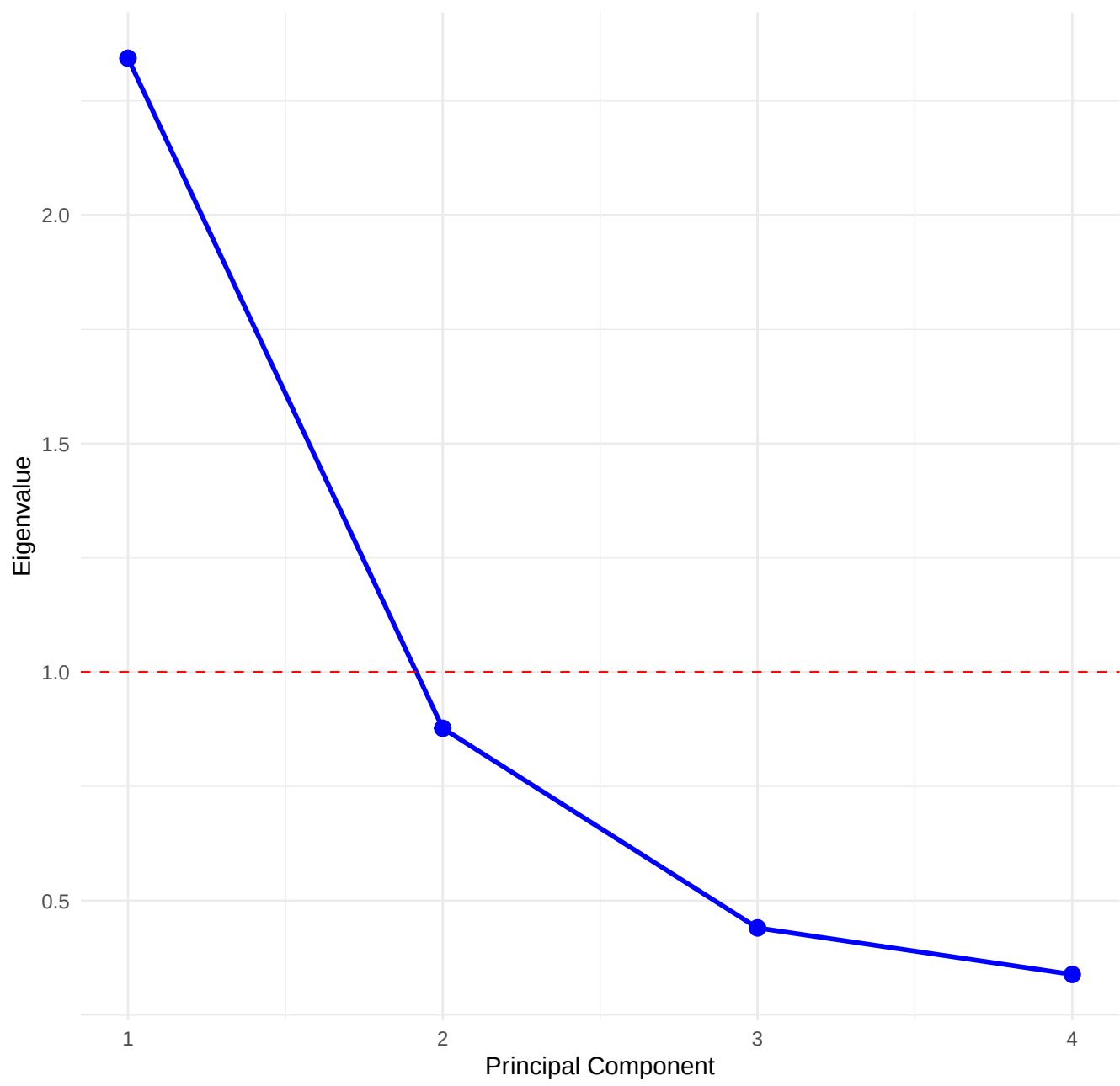
Scree Plot
