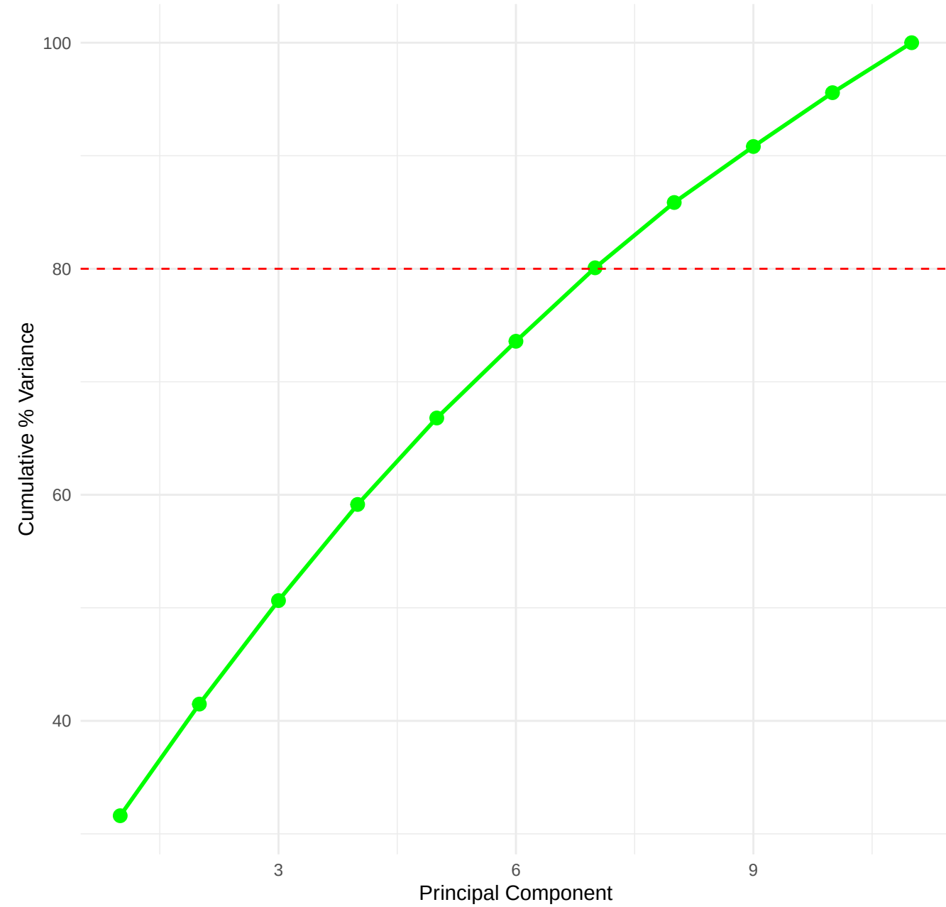
Cumulative Variance
