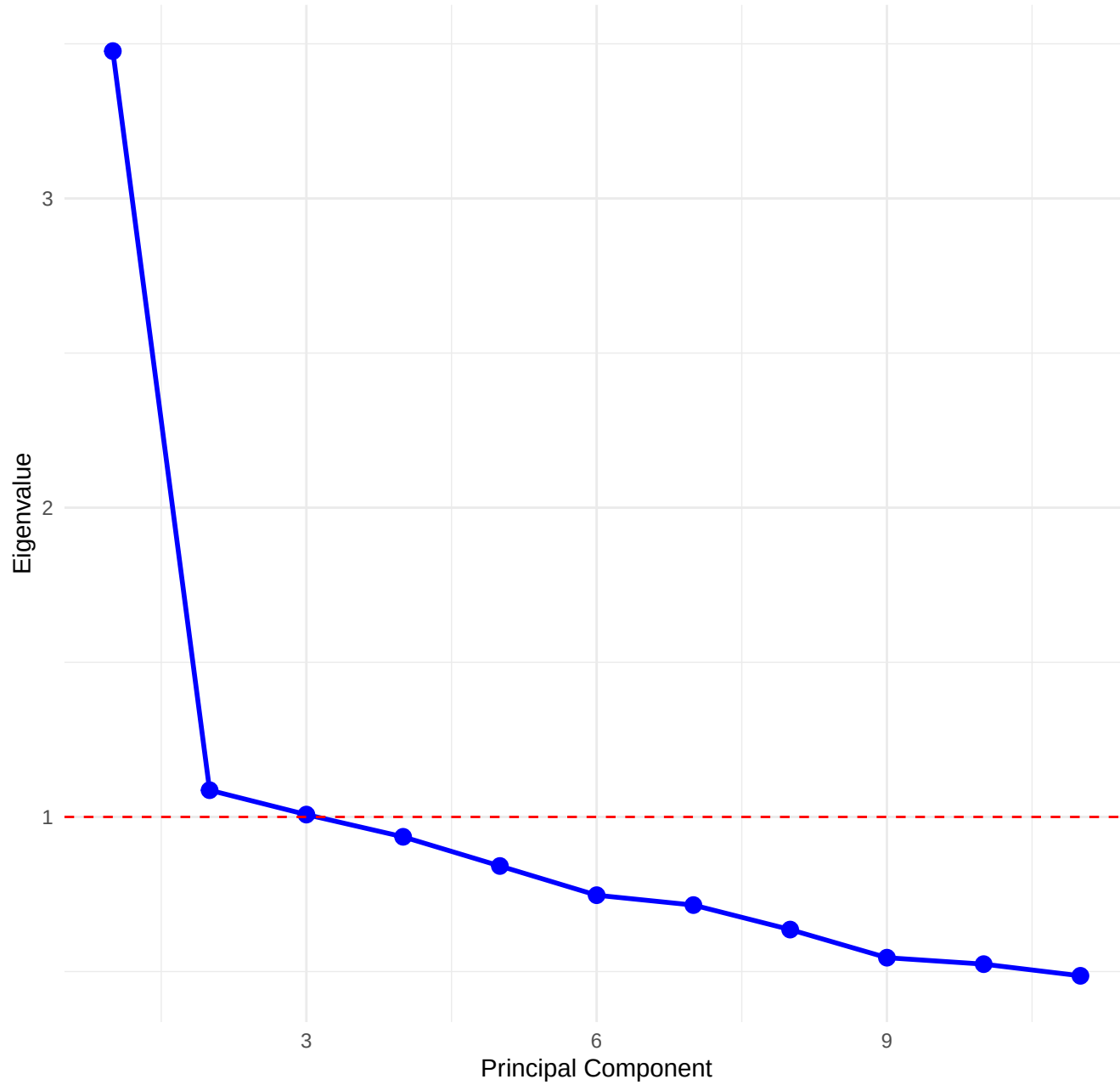
Scree Plot
