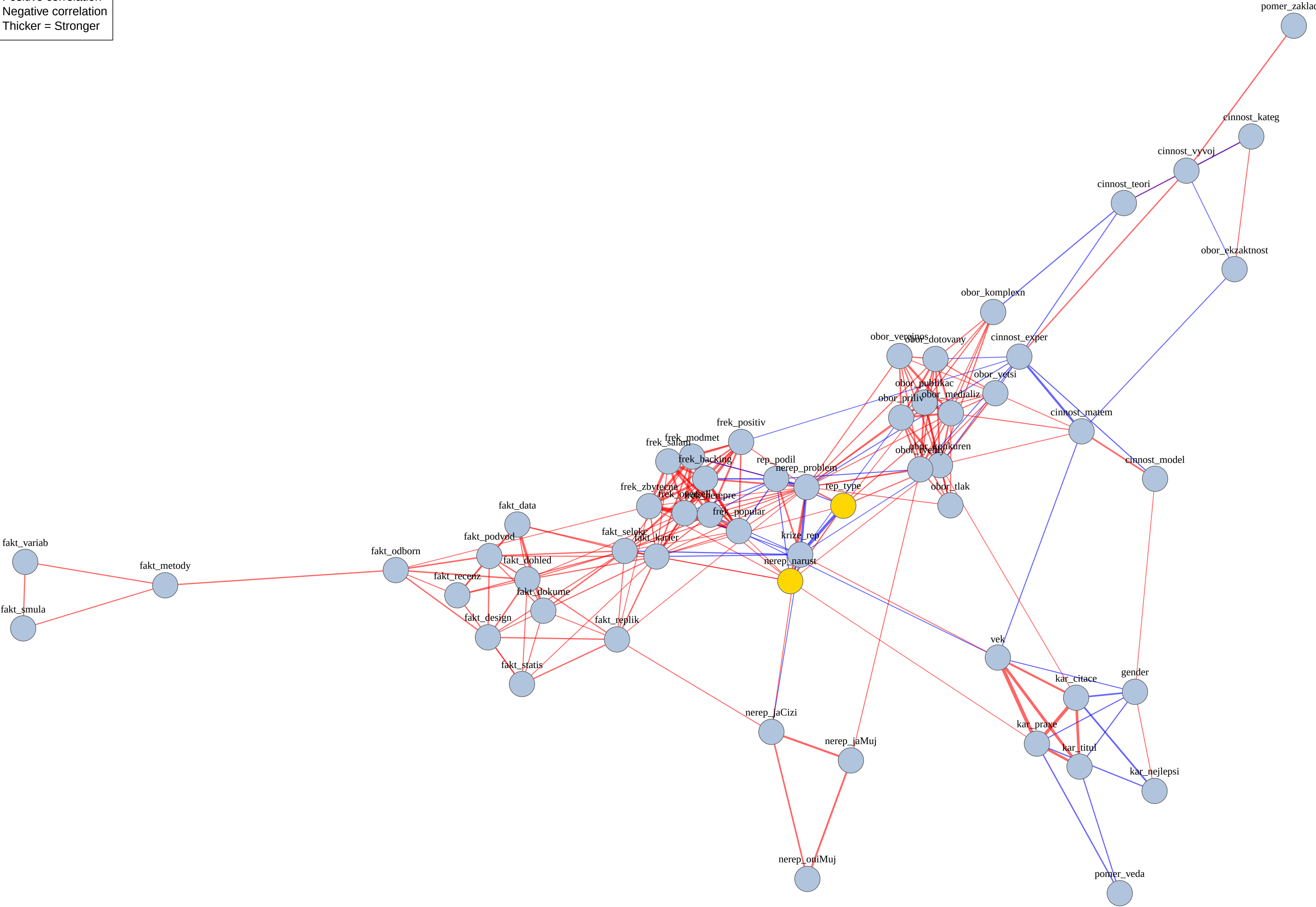
Correlation Network (Holm-corrected, Fruchterman-Reingold Layout)
