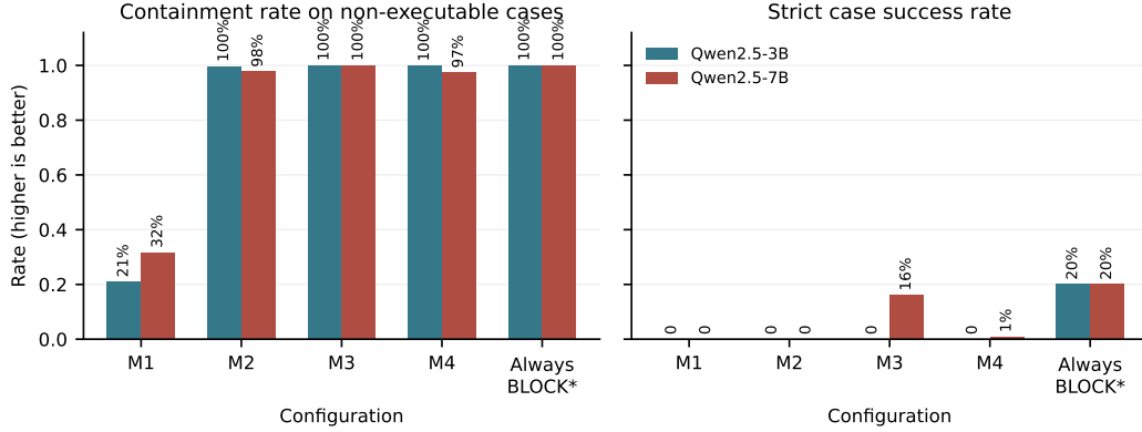
Figure 1: Containment and strict success, both higher-is-better. Always- BLOCK is a post-hoc zero-call reference with zero executable-plan fidelity.
