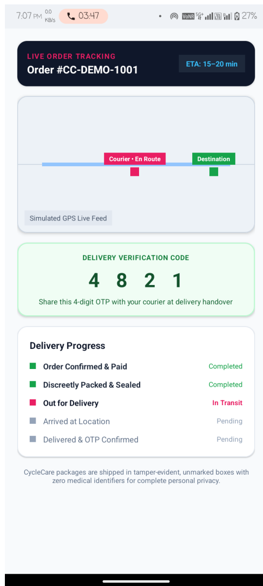
Figure: OrderTrackingActivity - Live Route Map & OTP 4821
