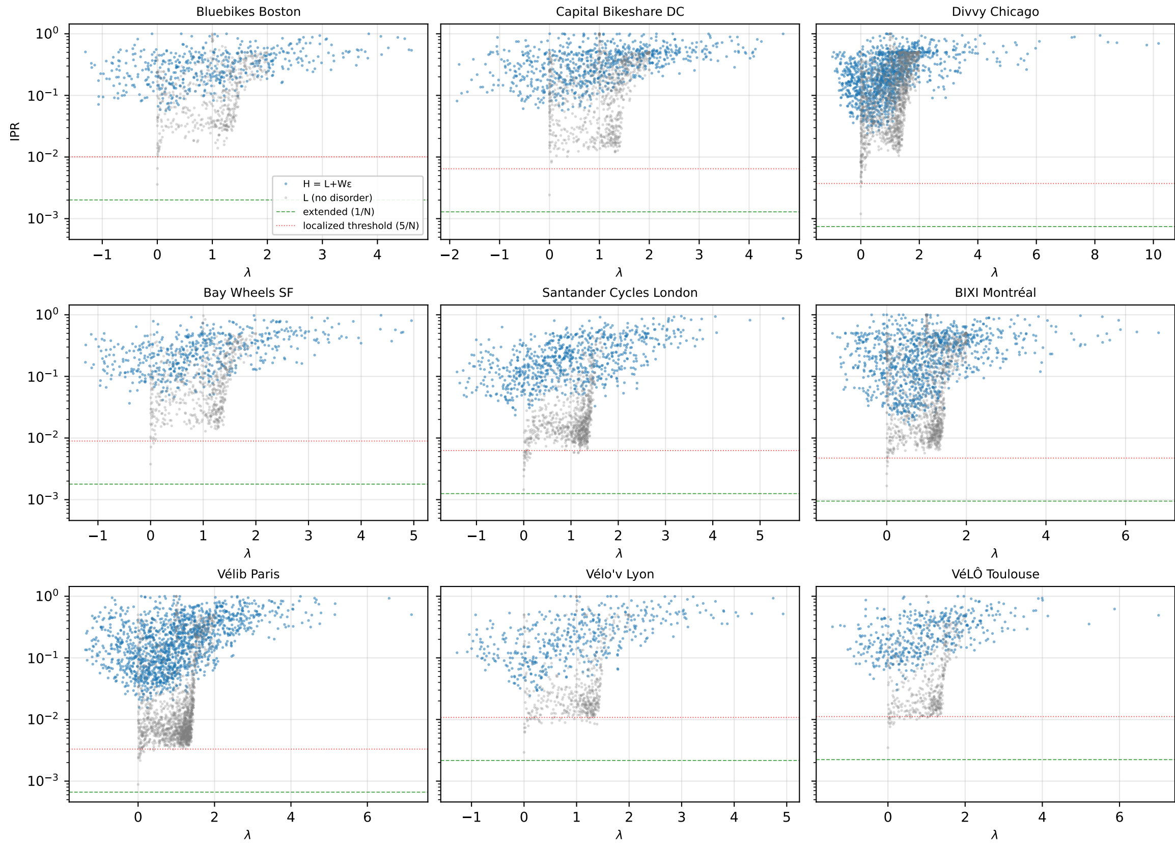
Anderson IPR vs energy on urban mobility graphs Above the 5/N red line: localized. At the 1/N green line: extended.
