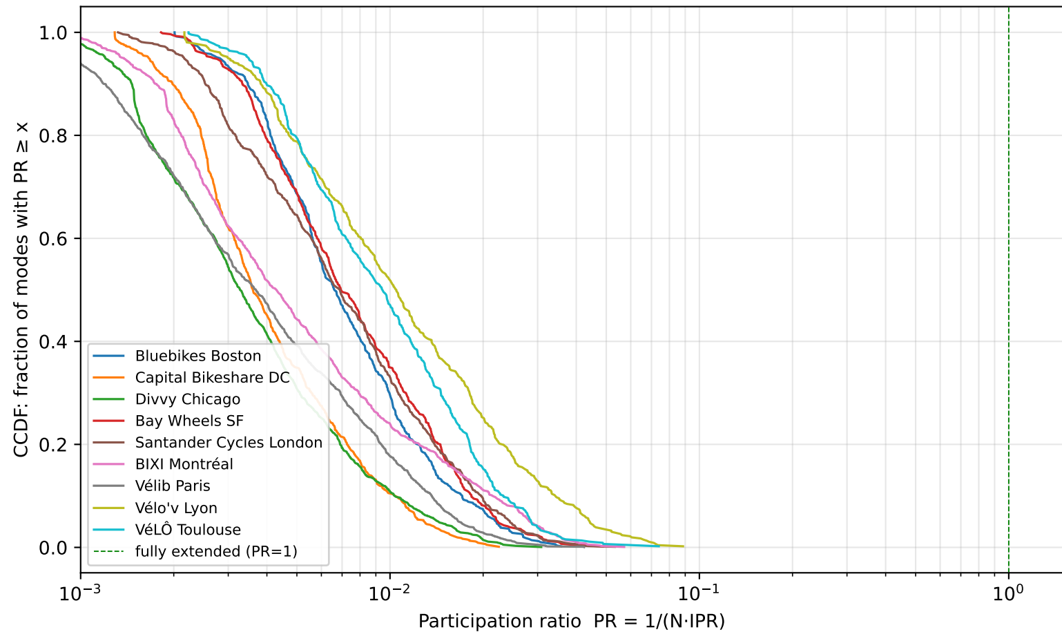
PR distributions — left mass = localized modes
