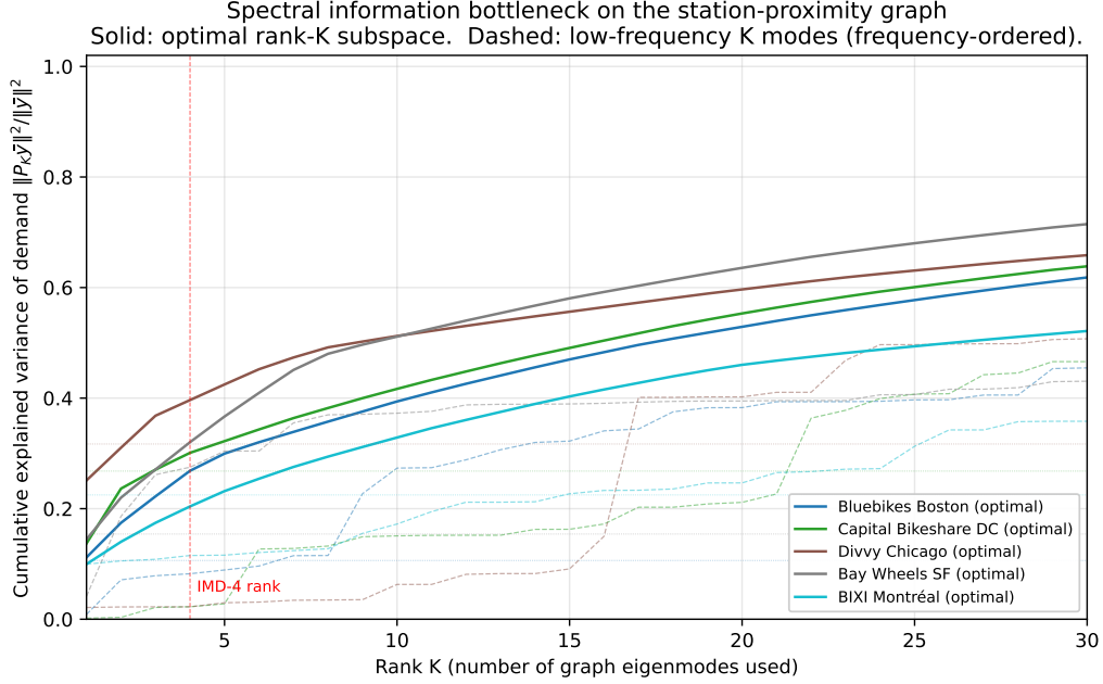
Figure 4. Spectral information bottleneck on the station-proximity graph. Solid lines report the optimal rank- K explained variance of demand (Eq. 16, top- K modes by demand power); dashed lines report the cumulative explained variance using the K lowest-frequency modes (natural frequency ordering). The vertical red line marks K = 4 , the rank of the IMD-4 subspace. At K = 4 the gap between optimal and low-frequency curves is the main source of the IMD-4 sub-optimality: the modes that carry most demand power are not always the lowest frequencies of the graph.
