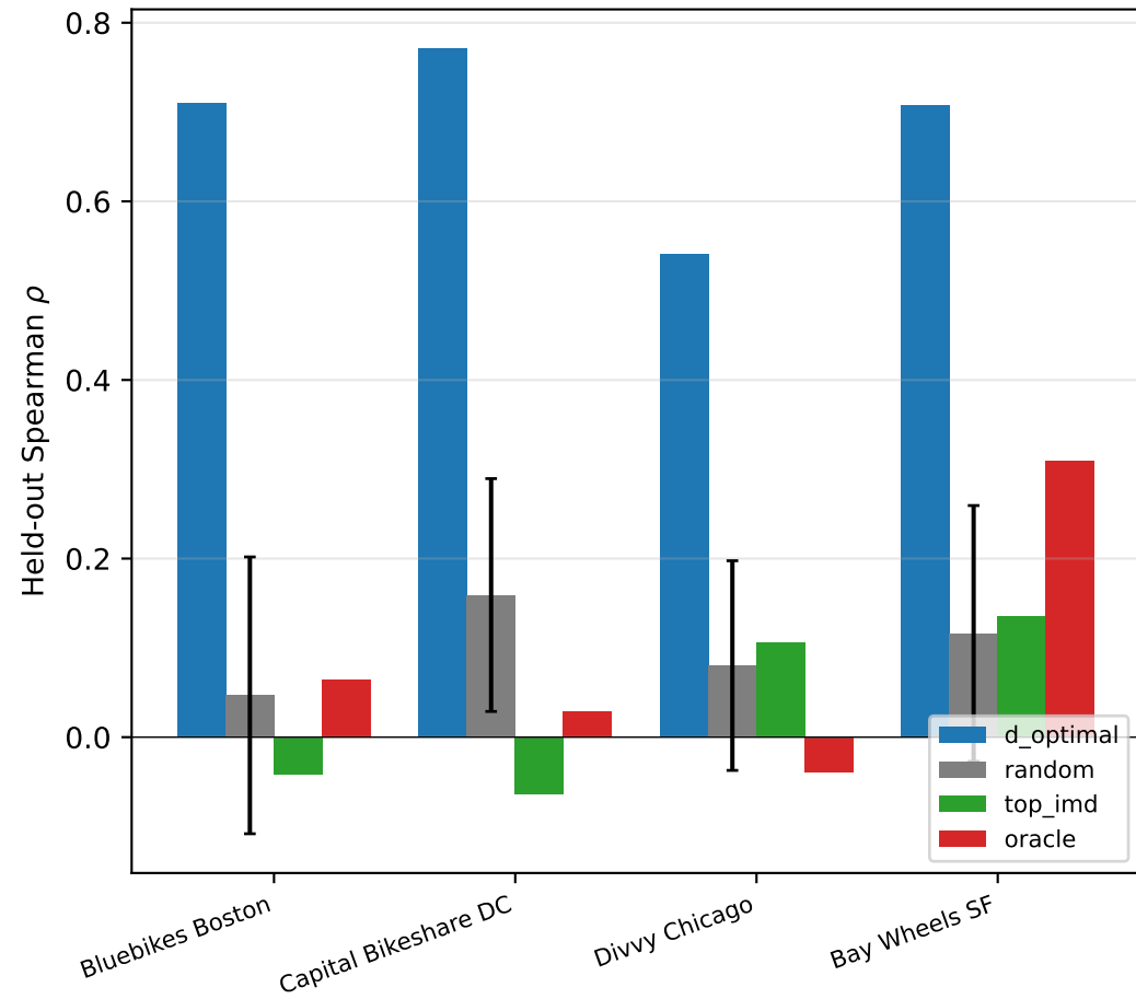
Siting-strategy comparison on the band-limited reconstruction task
