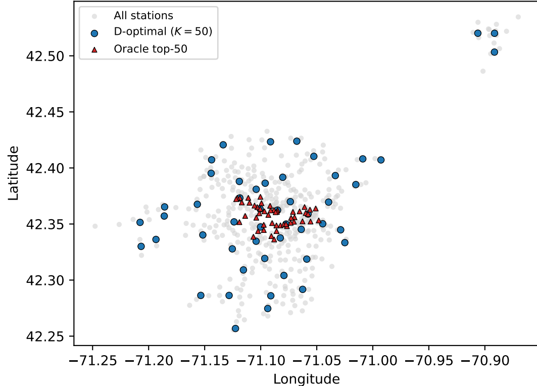
D-optimal vs oracle siting on Bluebikes Boston (N = 497)
