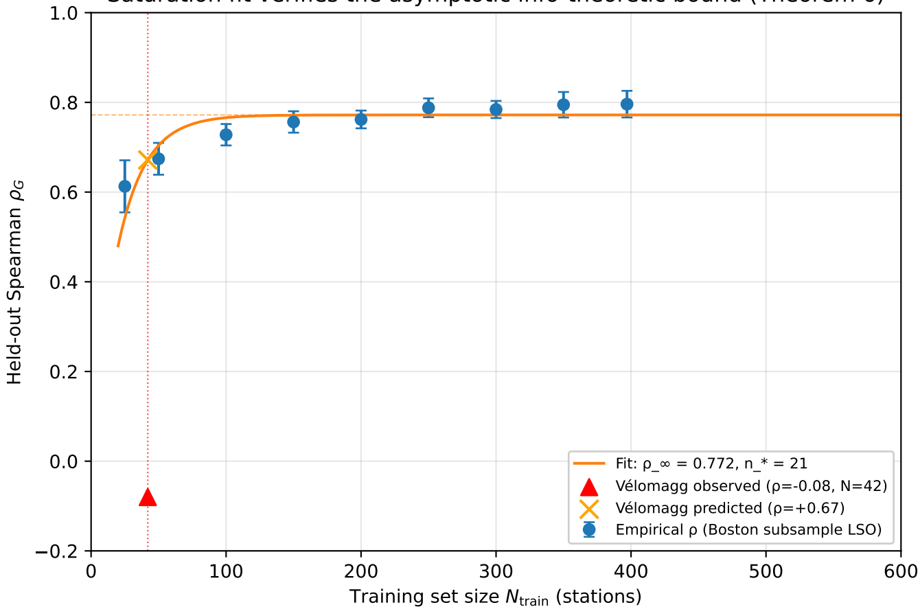
Empirical learning curve of IMD-augmented LSO on Boston Saturation fit verifies the asymptotic info-theoretic bound (Theorem 6)
