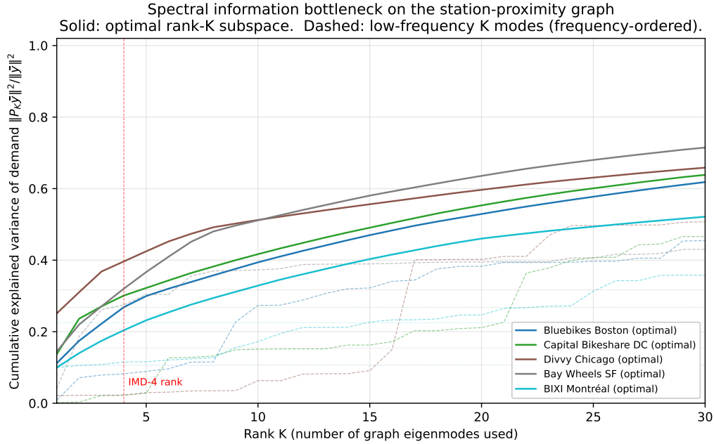
Figure 5. Spectral information bottleneck on the station-proximity graph. Solid lines report the optimal rank- K explained variance of demand (Eq. 15, top- K modes by demand power); dashed lines report the cumulative explained variance using the K lowest-frequency modes (natural frequency ordering). The vertical red line marks K = 4 , the rank of the IMD-4 subspace. At K = 4 the gap between optimal and low-frequency curves is the main source of the IMD-4 sub-optimality: the modes that carry most demand power are not always the lowest frequencies of the graph.
