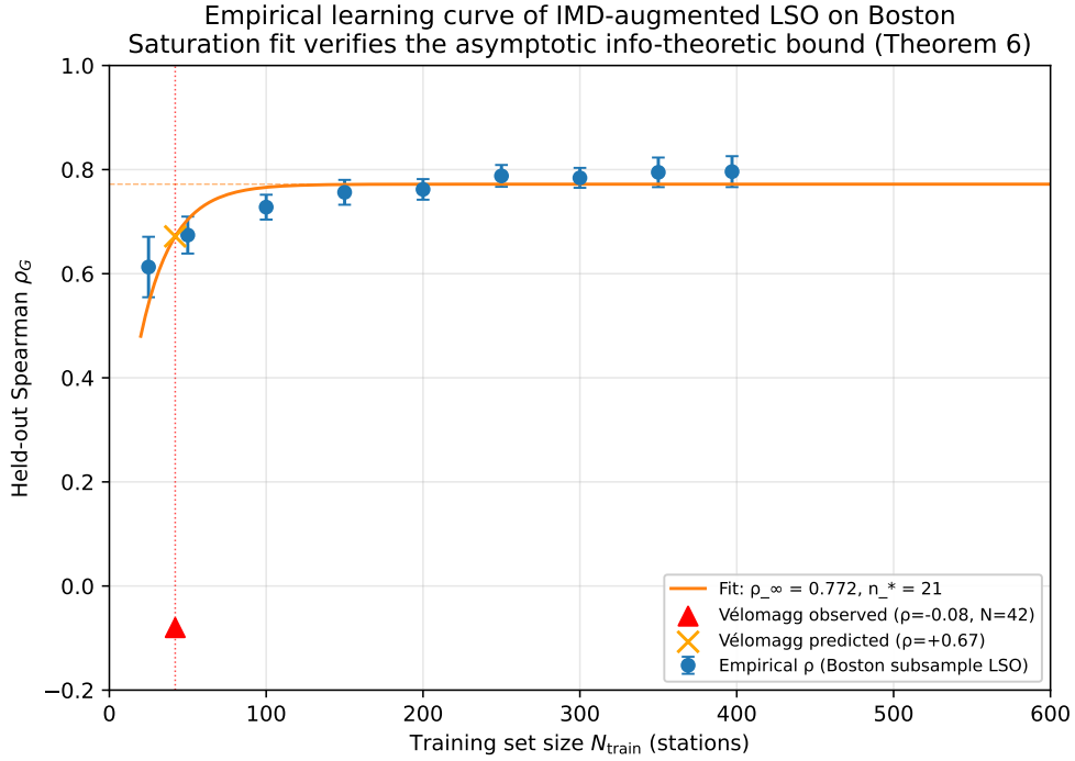
Figure 4. Empirical learning curve of the IMD-augmented LSO on Bluebikes Boston ( N \in \{25, \dots, 397\} training stations, 15 replications per N ). The fitted saturation \rho_G(N) = \rho_\infty(1 - e^{-N/n_*}) with \rho_\infty = 0.77 , n_* = 21 reaches 99% of the asymptote by N \approx 100 training stations. The Boston subsample at N = 25 stations achieves \rho = +0.61 — a key contrast with the VéloMagg LSO at N = 42 where \rho = -0.08 (red triangle). The gap of \sim 0.7 in Spearman \rho between the two N = 25 – 42 data points cannot be explained by sample size alone: at equal N on Boston the saturation curve already predicts \rho > +0.6 , against -0.08 observed on VéloMagg.
