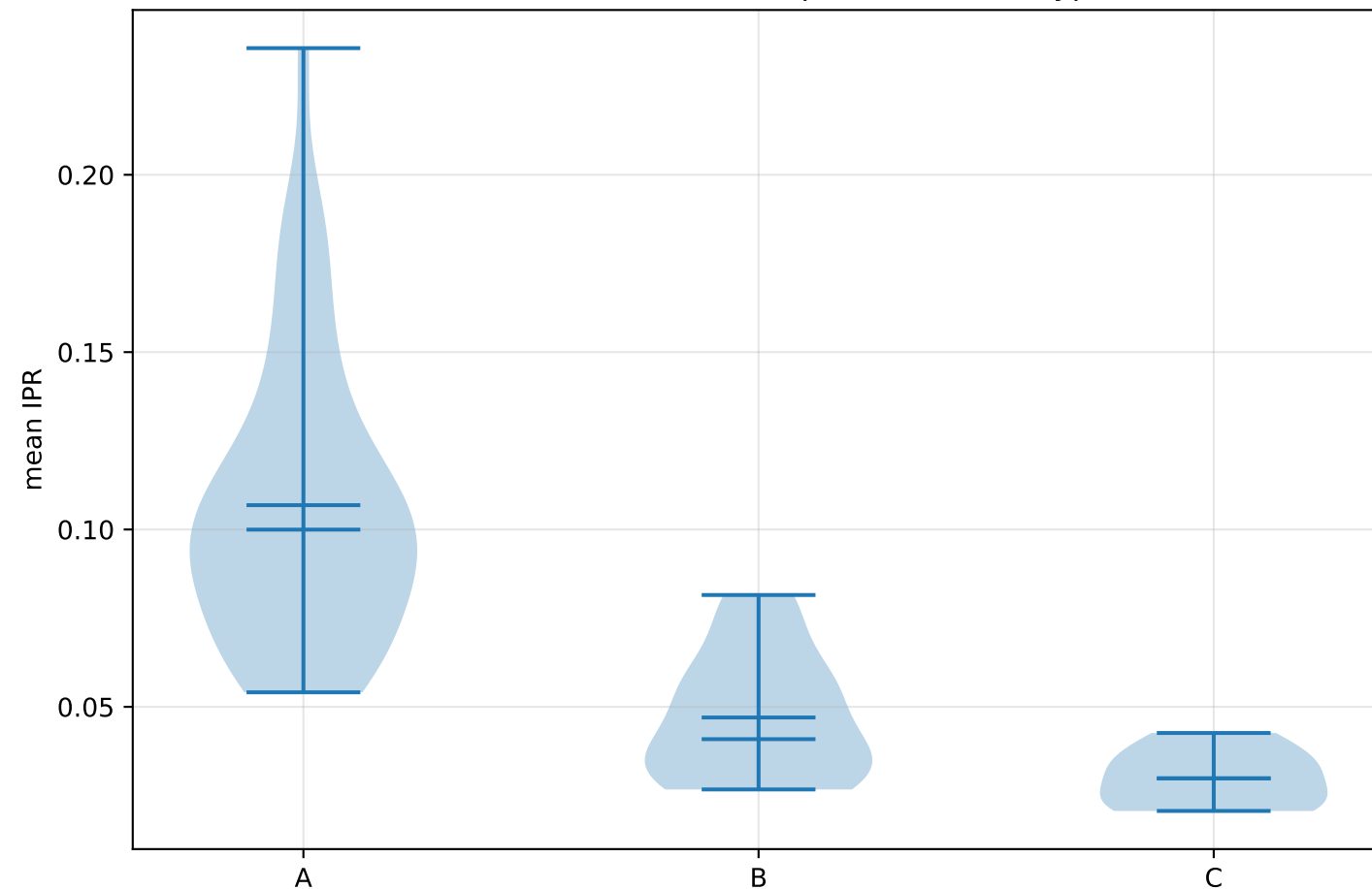
(b) Mean IPR distribution per discovered type
