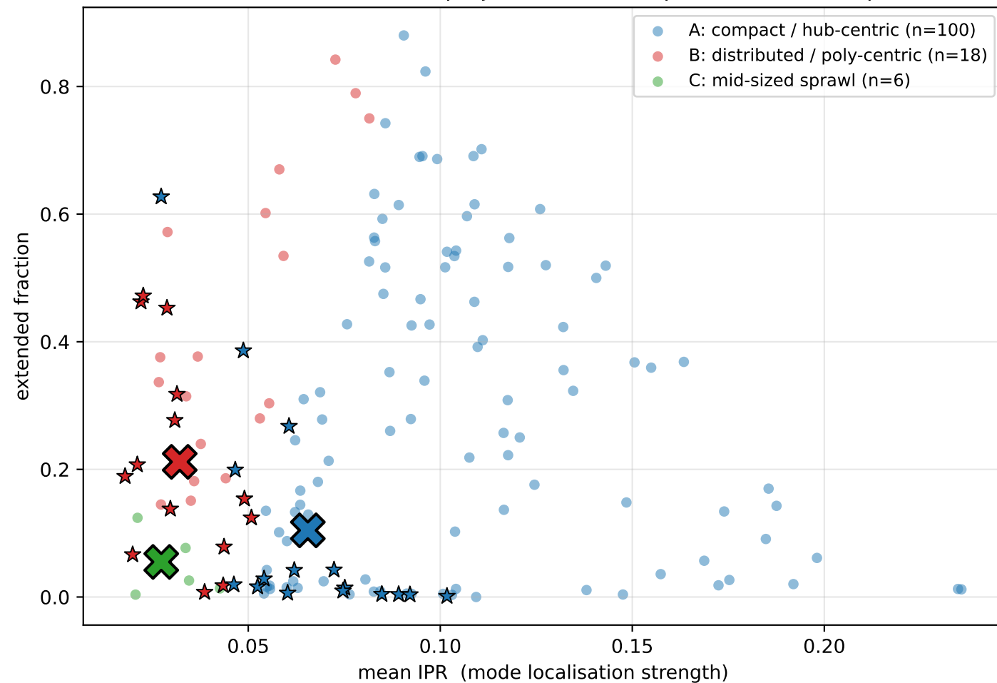
(a) Atlas-wide spectral taxonomy 124 bike-share networks projected onto the panel-discovered plane
