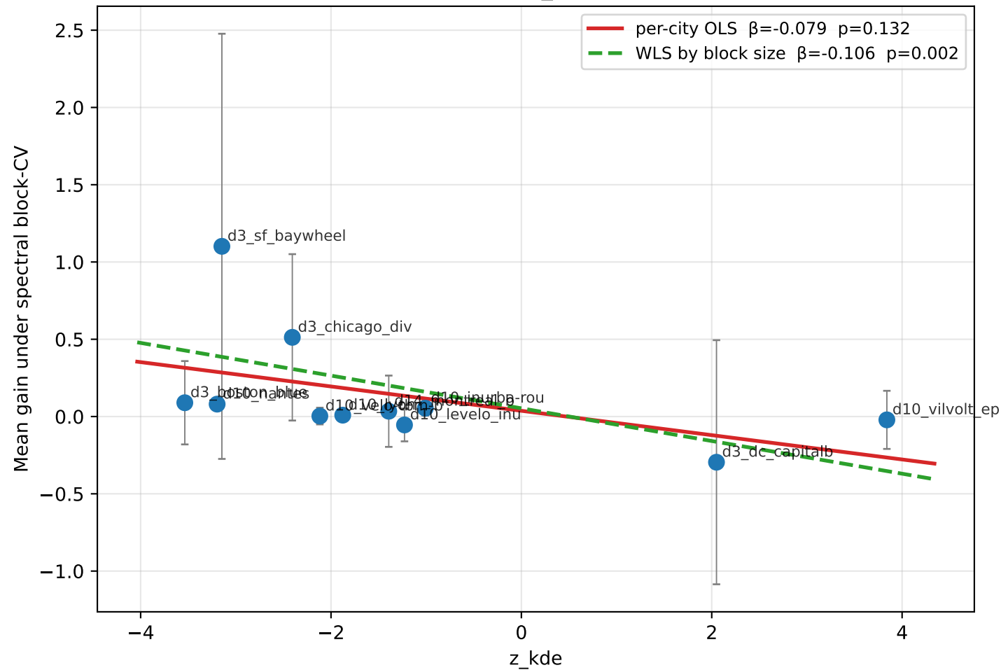
(a) Robust estimators of \beta(z\_kde) on the block-CV gain
