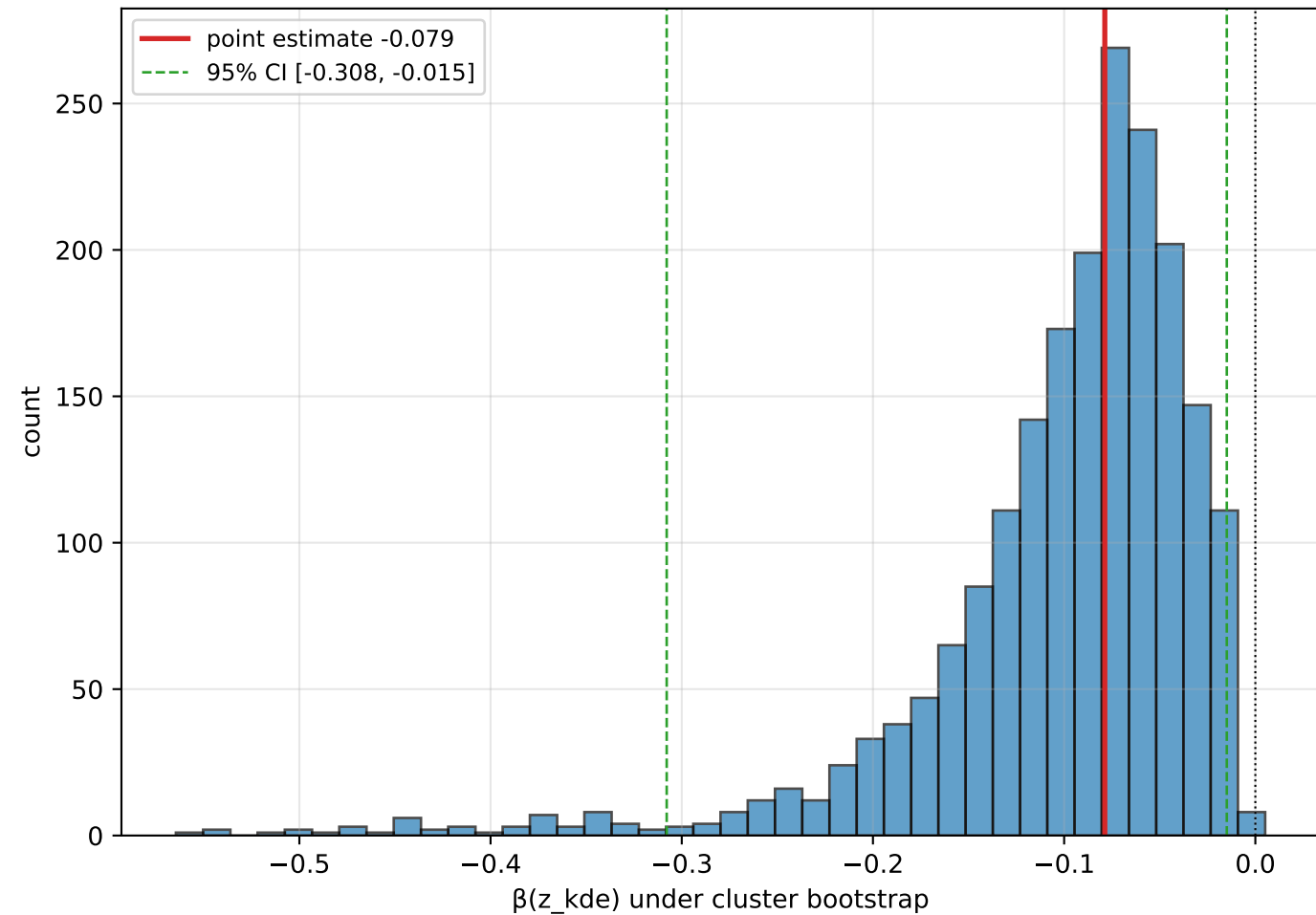
(b) Cluster bootstrap ( N\_boot=2000 ) fraction \beta < 0 = 100\% two-tailed p = 0.0010
