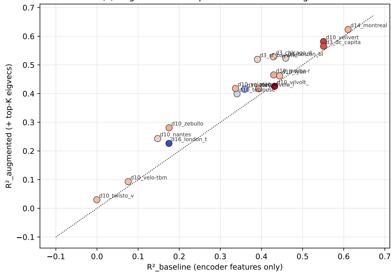
(c) Augmentation helps when above the diagonal
