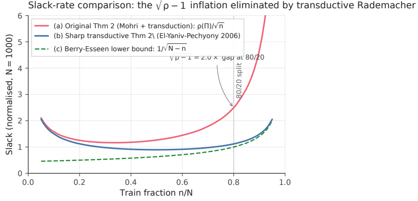
Figure 1: Slack-rate comparison illustrating Theorem 11’s improvement over a naive Mohri-routed proof. Plotted as a function of the train fraction n/N (at N = 1000 , normalised so the Berry–Esseen lower bound equals 1 at n/N = 0.8 ): (a) original Theorem 2 slack \rho(\Pi)/\sqrt{n} , (b) sharp transductive Theorem 2 slack \sqrt{1/n + 1/u} via El-Yaniv–Pechyony 2006, and (c) Berry–Esseen minimax lower bound 1/\sqrt{N-n} . The multiplicative gap between (a) and (c) is exactly \sqrt{\rho(\Pi) - 1} ( = 2.0\times at the standard 80/20 split), eliminated by the transductive Rademacher upgrade; (b) and (c) differ only by a slow constant. Generated by experiments/d02_slack_comparison_figure.py .
