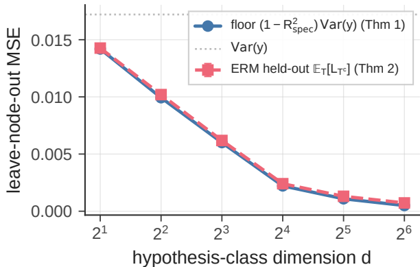
Thm 1 floor vs. ERM held-out error (synthetic graph)
