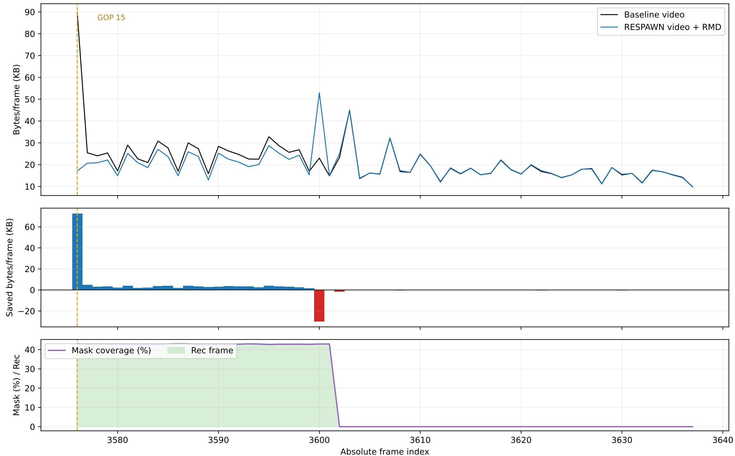
fm6_00: per-frame byte behavior across complete GOP(s) 15
