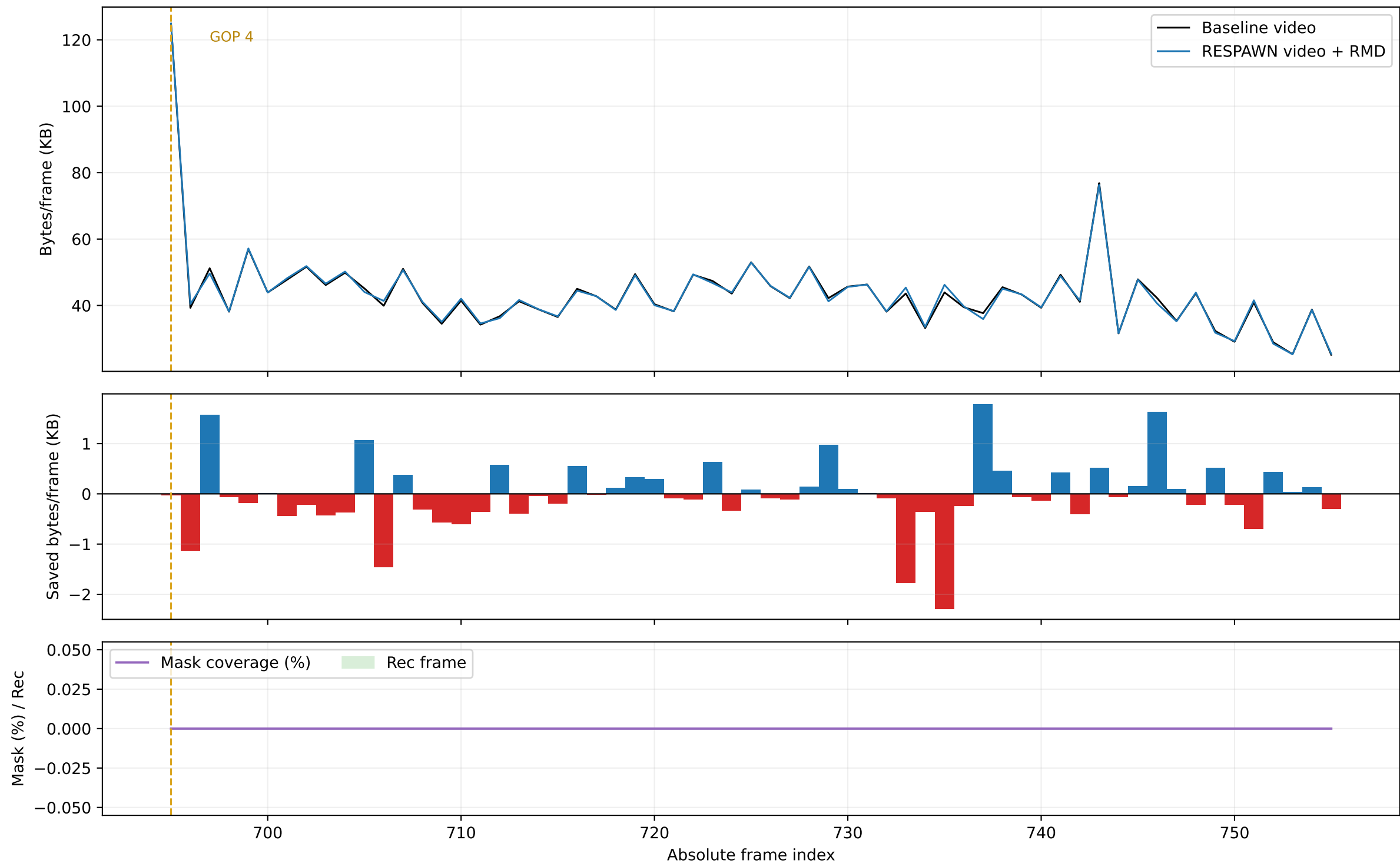
fm6_03: per-frame byte behavior across complete GOP(s) 4
