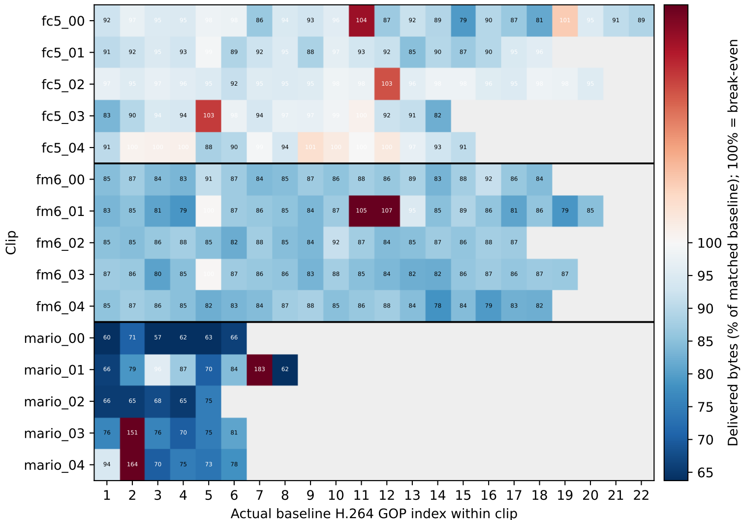
Per-GOP delivered bandwidth relative to baseline
