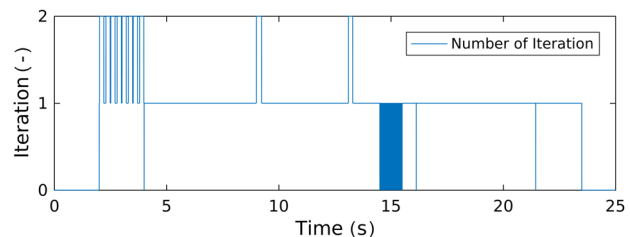
Fig. 9 Number of iterations for solving the forward kinematics during experiment
