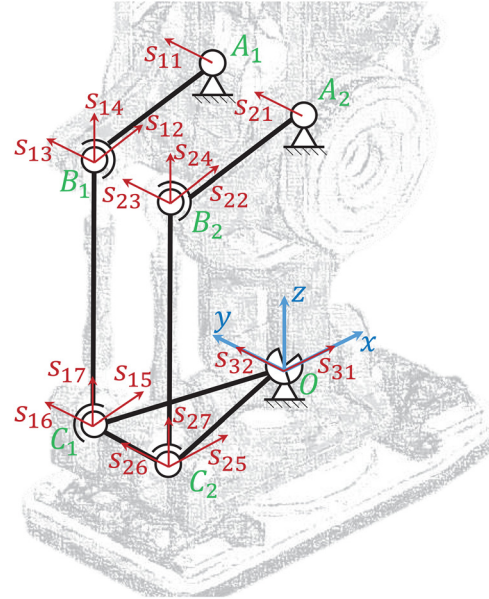
Fig. 2 The ankle's schematic representation
