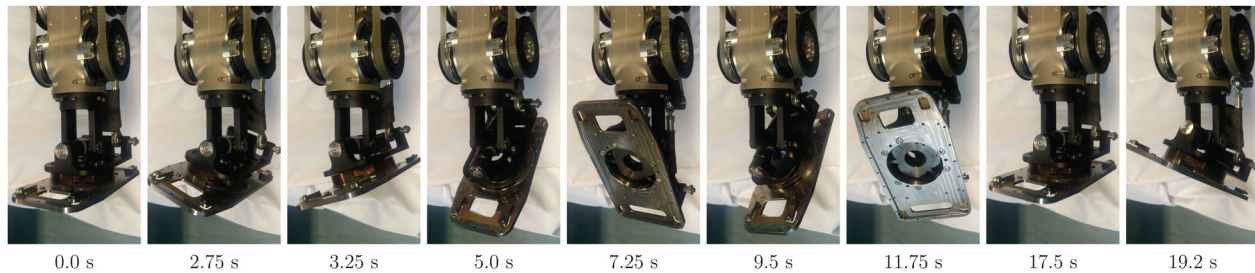
Fig. 11 Snapshots of the four experimental tests 5
