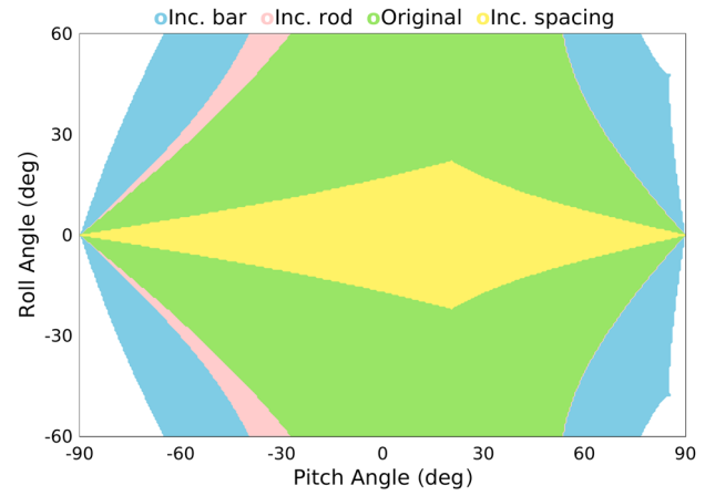
Fig. 4 The ankle workspaces with respect to only the mechanism geometry, are illustrated in green for the default equal dimensions, in blue by increasing the motor bar length, in pink by increasing the rod length and in yellow by increasing the spacing between the two rods, respectively
