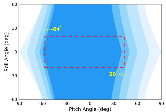
Fig. 5 The workspace of the proposed ankle illustrated by different motor limits with the lower limit varying from -90 to -60 deg and the upper limit varying from 90 to 40 deg. The red box represents the desired workspace. Therefore, the minimum required motor limits are [-64, 50] degree.
