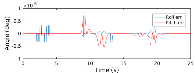
Fig. 8 Roll and pitch angle errors between the input references and the resultant ones after the IK-FK computation
