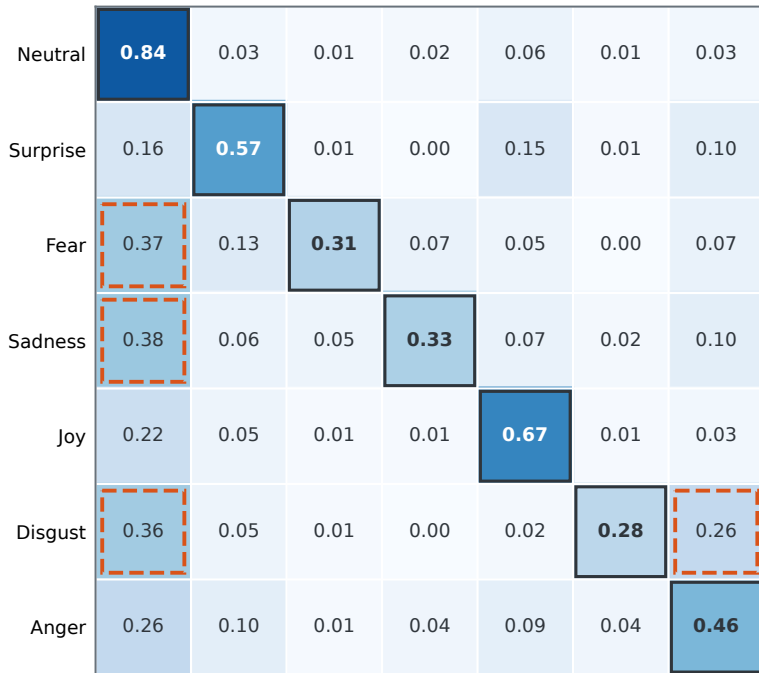
Ground-Truth Label
