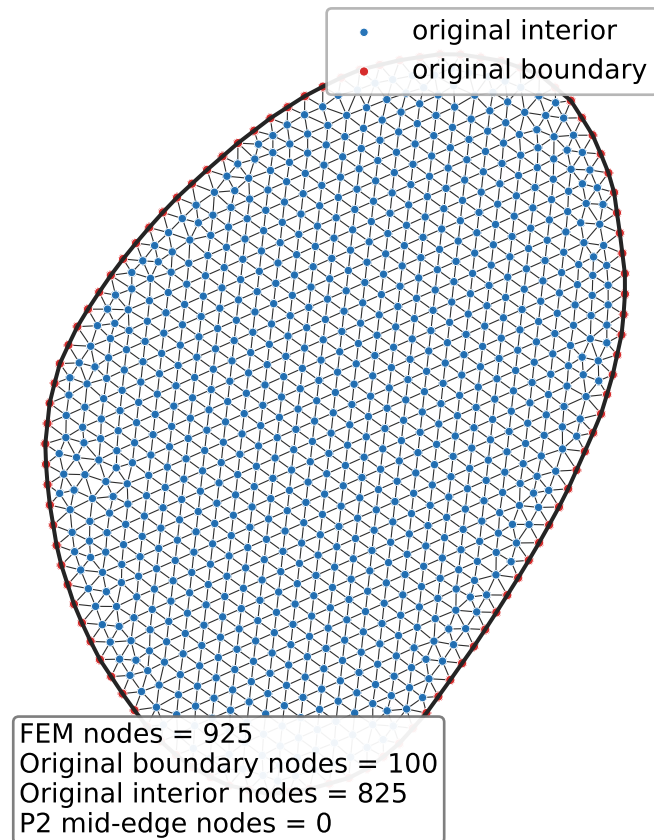
Transolver Input Point Cloud
