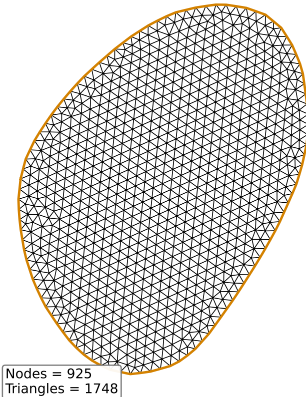
FE Mesh
