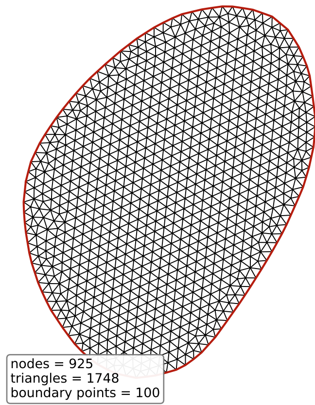
Subdomain FE Mesh
