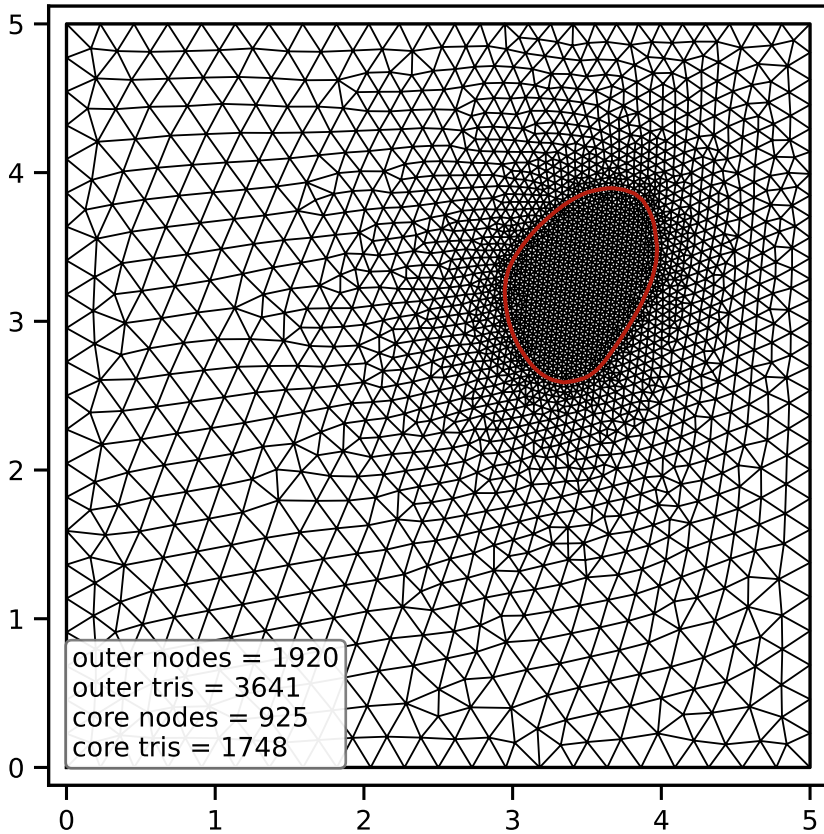
Whole Plate Mesh (Core Reinserted)
