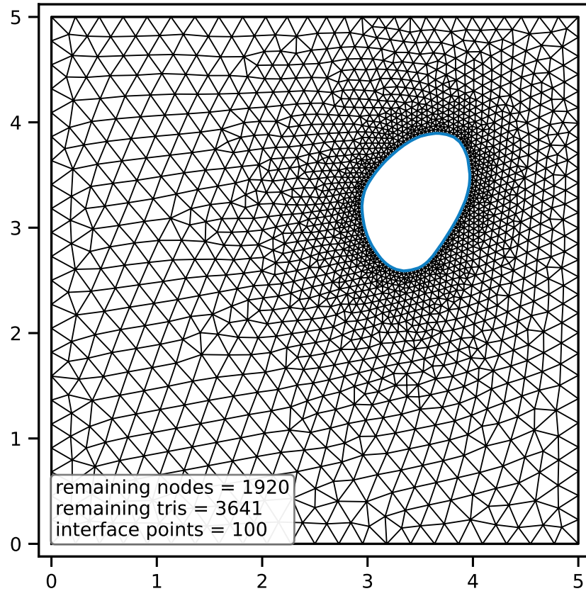
Outer FE After Removing Core
