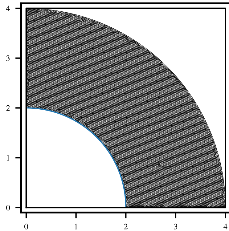
Outer Domain Mesh
