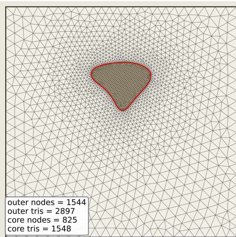
Whole Plate Mesh (Core Reinserted)
