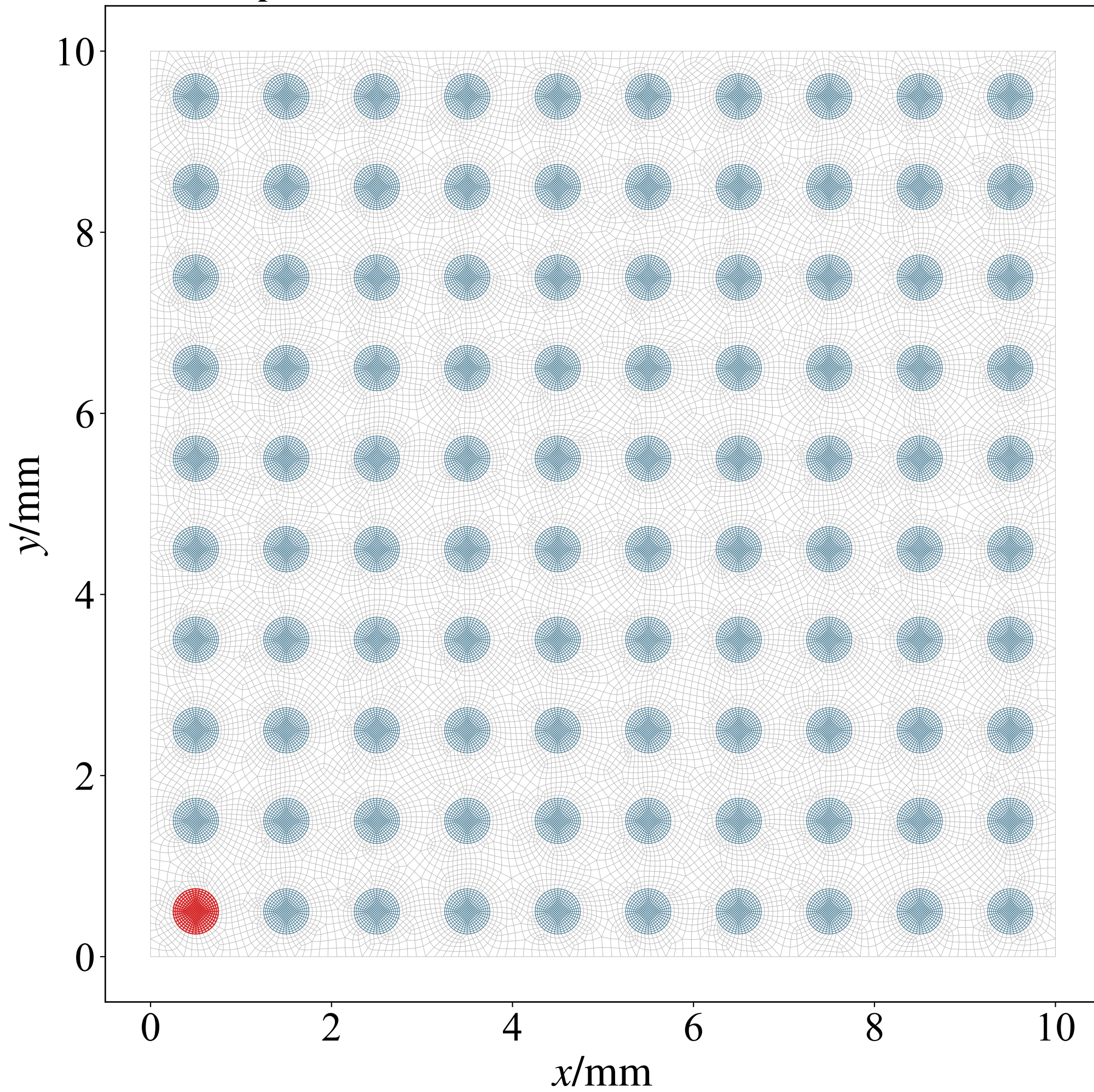
Complete Bottom Cross-Section: 100 Fibers and Matrix
