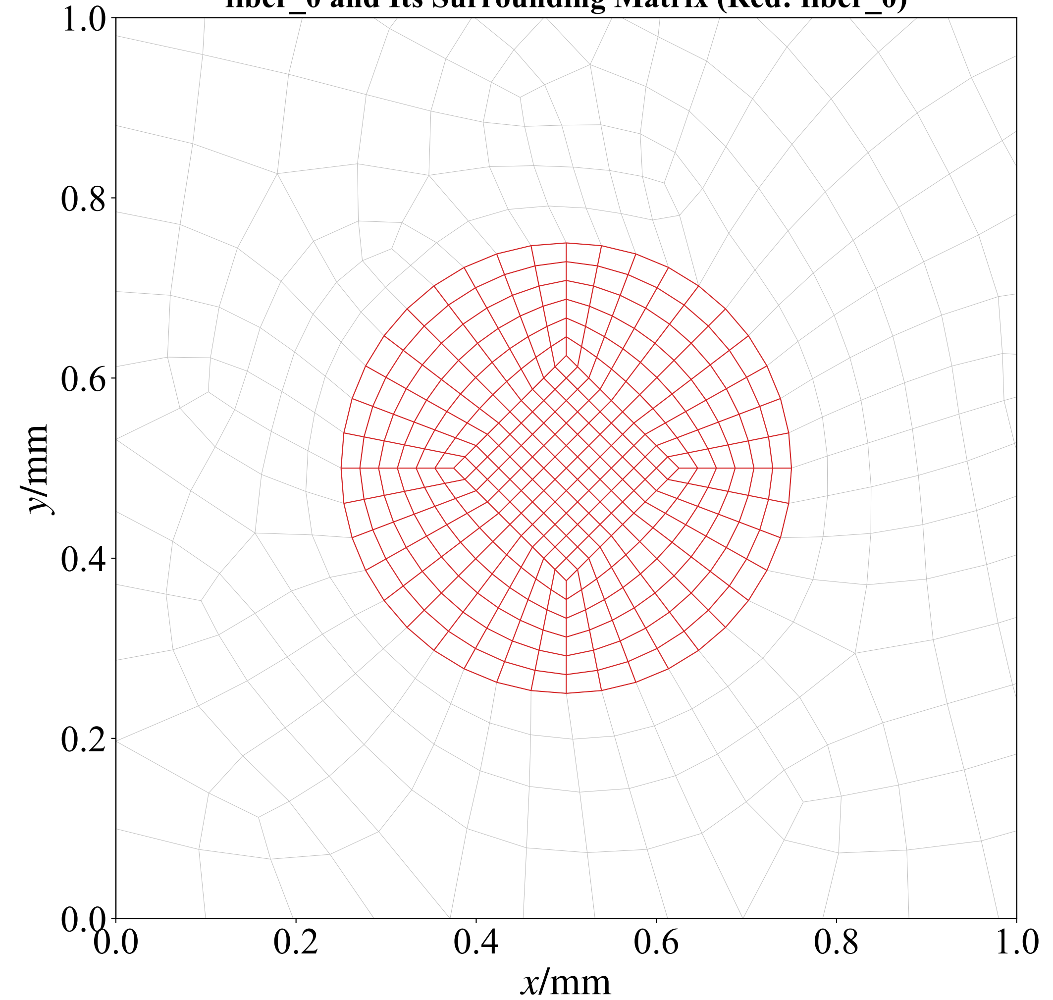
fiber_0 and Its Surrounding Matrix (Red: fiber_0)
