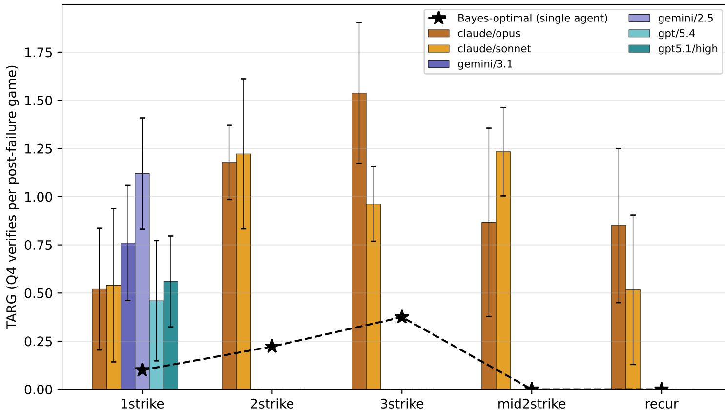
Observed LLM TARG vs Bayes-optimal verify rate (prior Beta(1,1), verify cost=1, death penalty=4.0)
