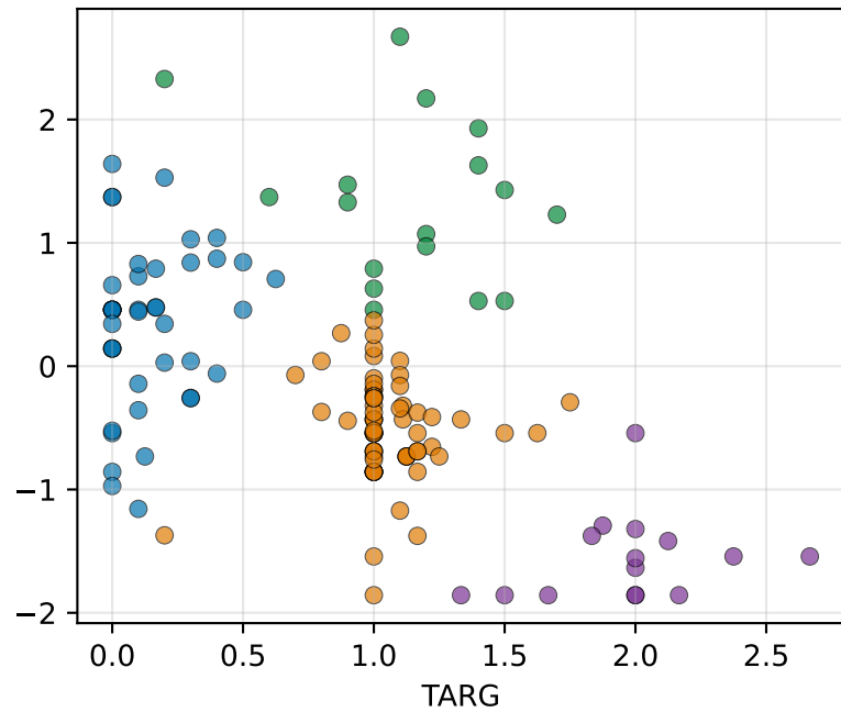
k-means silhouette=0.530
