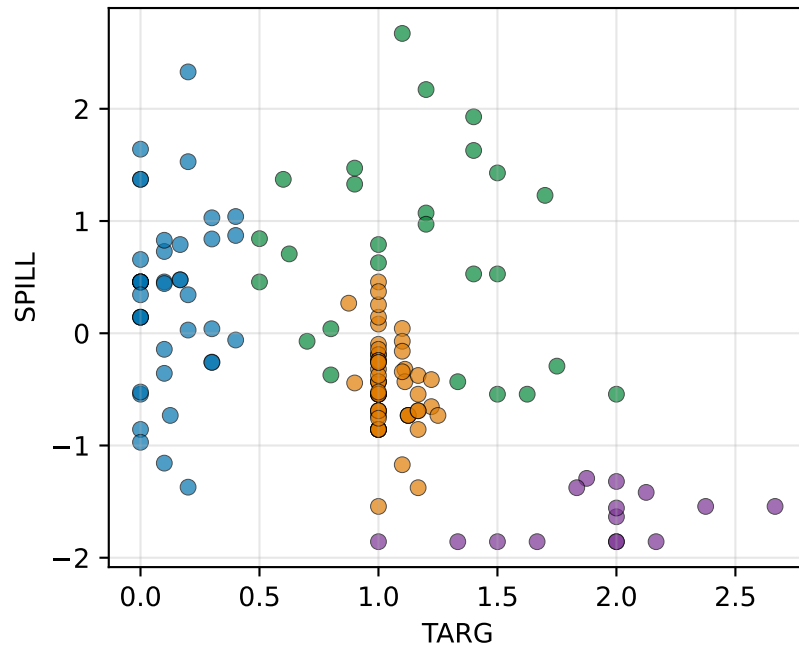
GMM (full cov) silhouette=0.451
