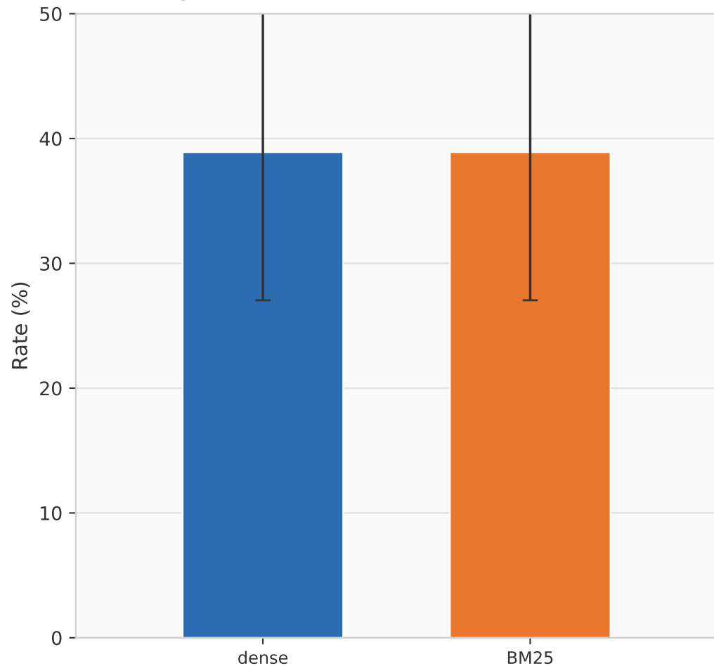
a gold-hit@5 (retriever recall, n=54)
