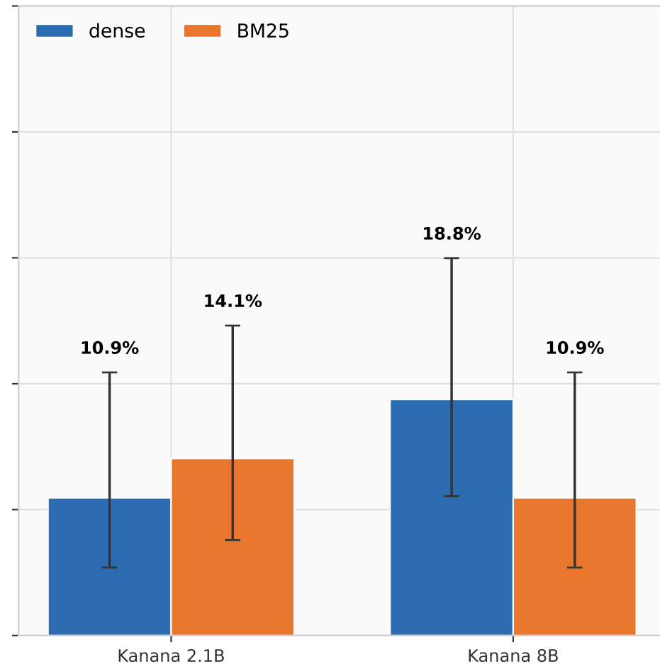
b contains-pass: dense vs BM25 (advisory, n=64)
