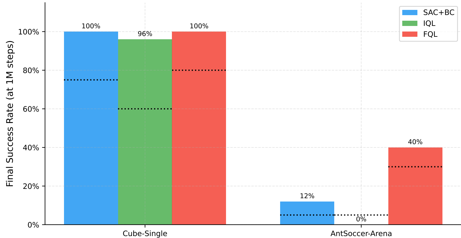
Final Success Rate Comparison (dotted = target)
