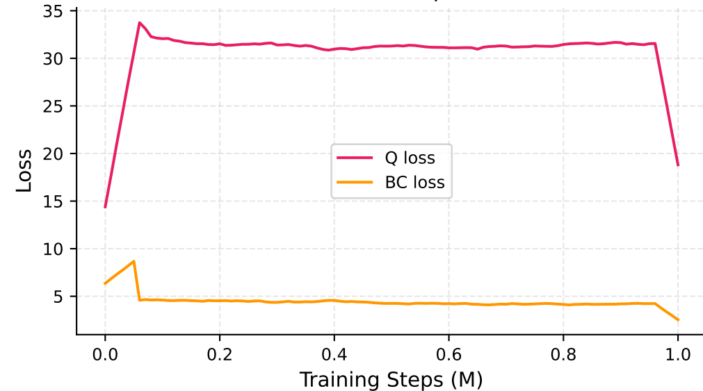
Actor Loss Components
