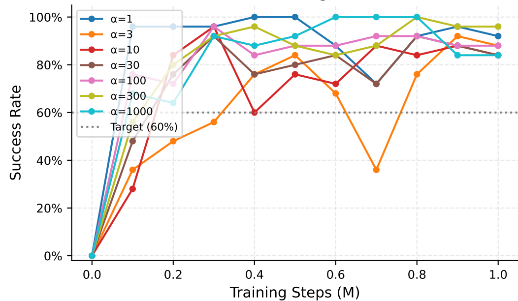
Cube-Single
