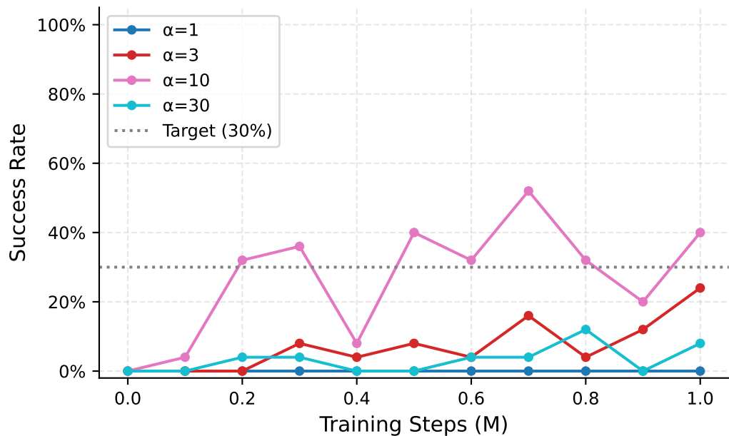
AntSoccer-Arena
