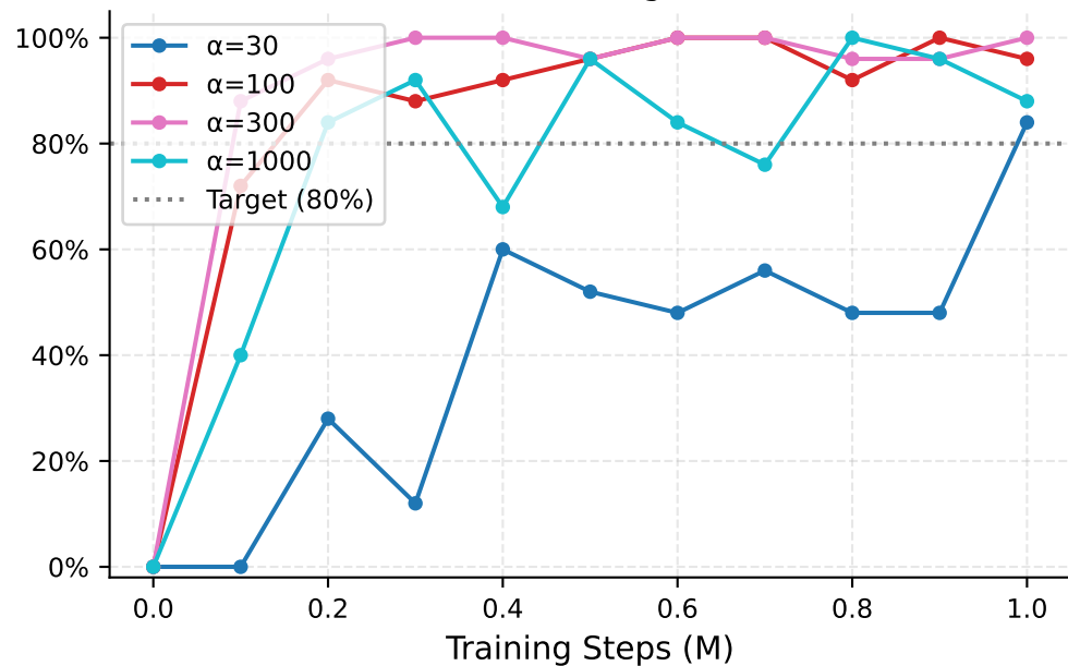
Cube-Single
