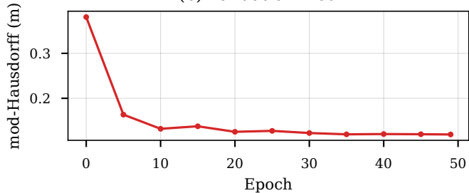
(b) Validation mod-H
