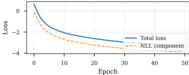
(a) Training Loss Components
