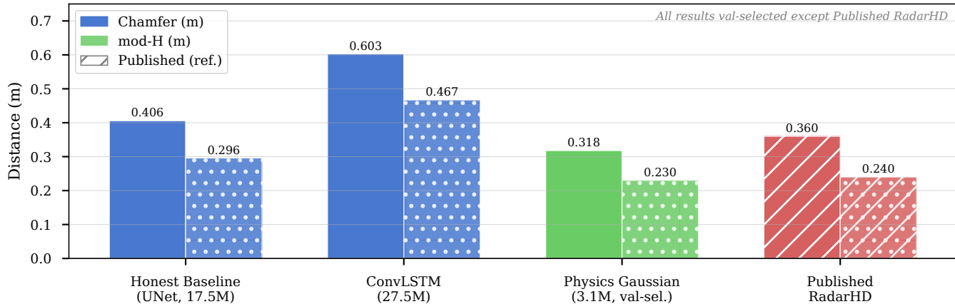
Model Comparison — Test Set (lower is better)
