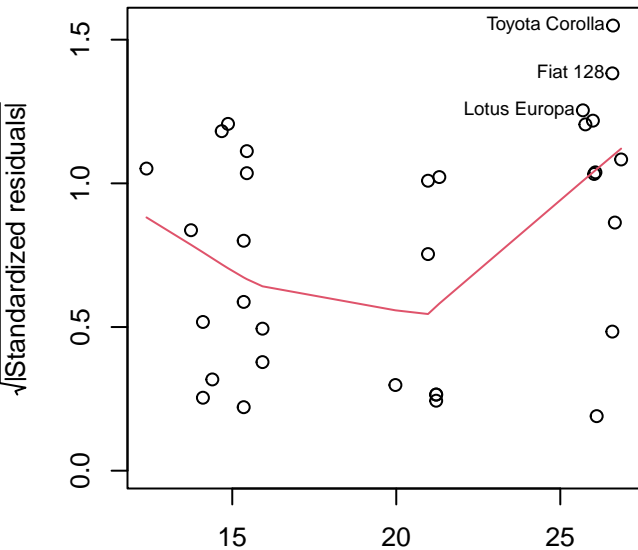
Scale-Location
