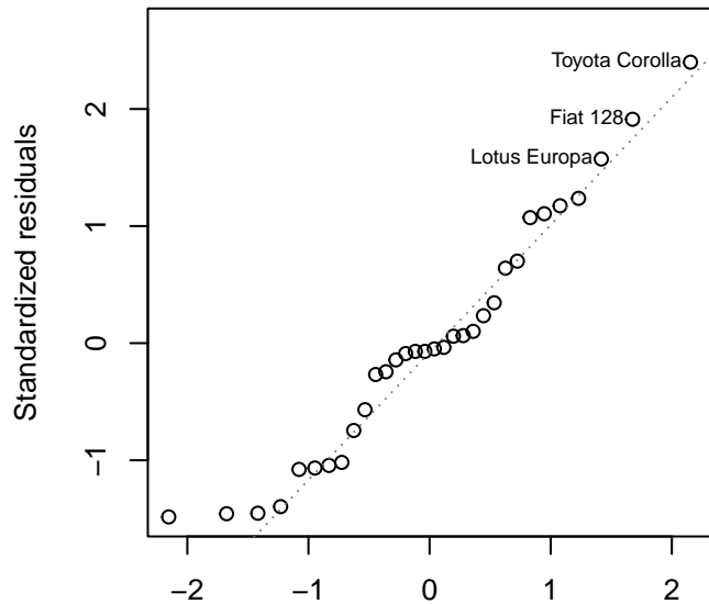
Q-Q Residuals
