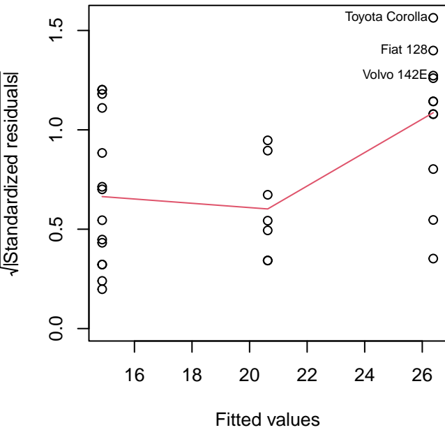
Scale-Location
