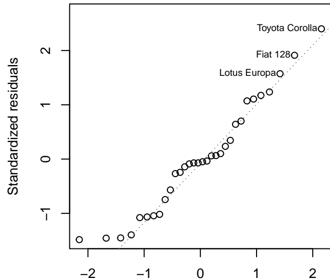
Q-Q Residuals
