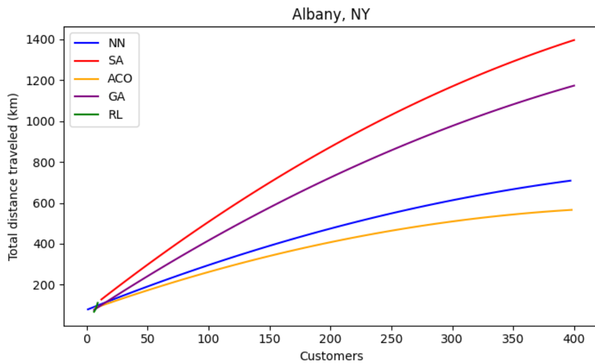
Fig. 1. 400 customers across 4 trucks with 100packages/truck(max. 100 customers/TSP)
