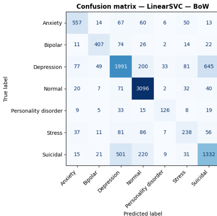
FIGURE 9.3 – Matrice de confusion — LinearSVC + BoW (Diogo)
