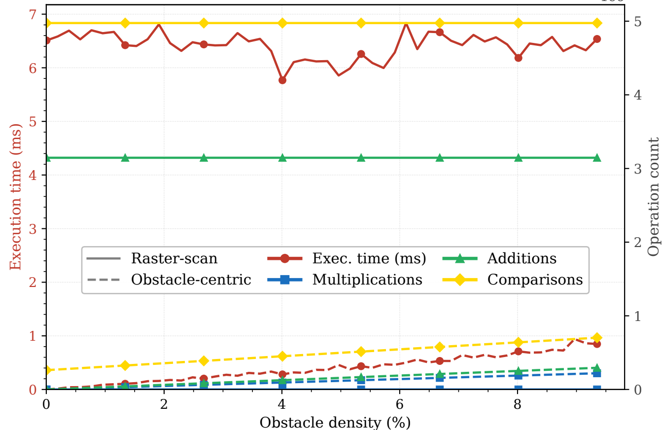
Raster-Scan vs. Obstacle-centric · 512×512 map, 3×3 kernel
