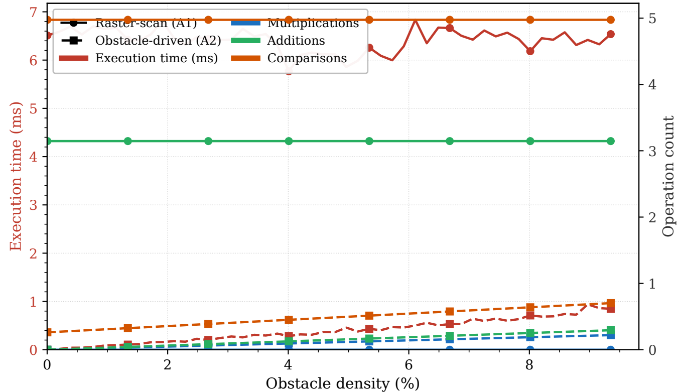
Raster-Scan vs. Obstacle-Driven — 512×512 map, 3×3 kernel
