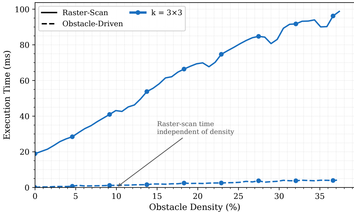
Execution Time: Raster-Scan vs. Obstacle-Driven — 512x512 Map
