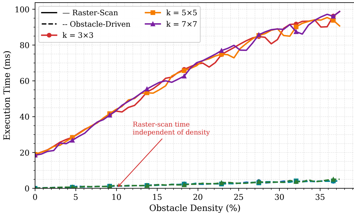
Raster-Scan vs Obstacle-Driven Inflation — 512x512 Map
