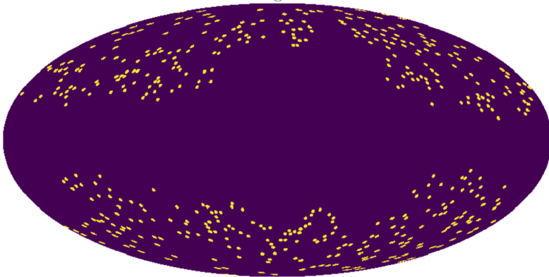
Lone Blazar Map, r_{\text{region}} = 1.0^\circ , N_{\text{bl}} = 463
