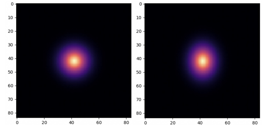
(a) Unlensed
