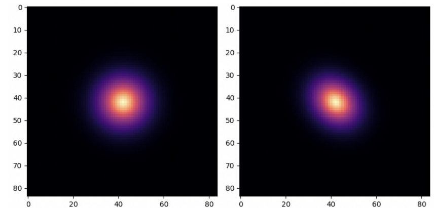
(e) \kappa
