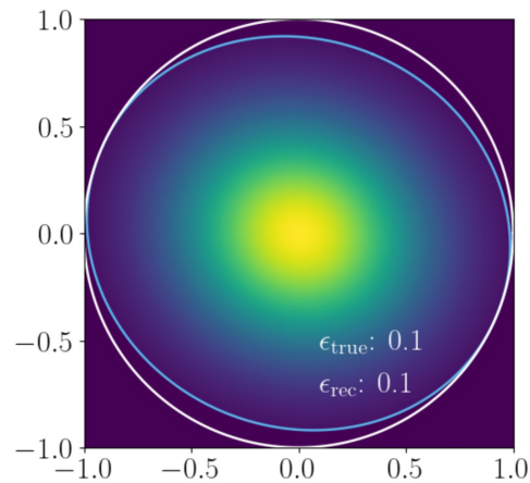
Convolution:
