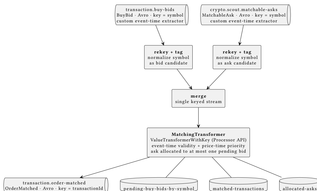
Figure 13: Transaction matching topology: the bid and ask streams are re-keyed to a common symbol, merged, and matched by a custom ValueTransformerWithKey over three persistent stores, emitting transaction.order-matched keyed by transactionId
