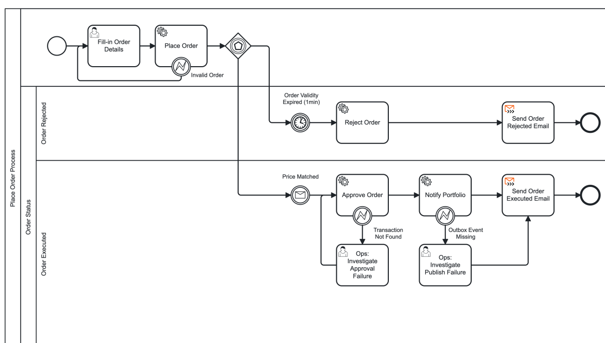
Figure 8: Place order BPMN process with Kafka-backed matching, timeout handling, downstream publication, and operations tasks that loop the resolved instance back into the happy path (ADR-0035)
