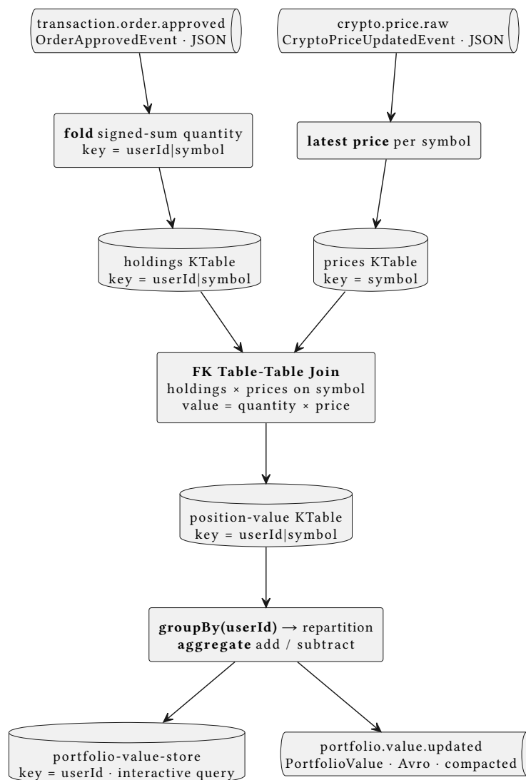
Figure 14: Portfolio valuation topology: approved orders and prices become KTables, a foreign-key table-table join yields per-position values, and a groupBy(userId) repartition aggregates them into the queryable portfolio-value-store and the compacted portfolio.value.updated topic
