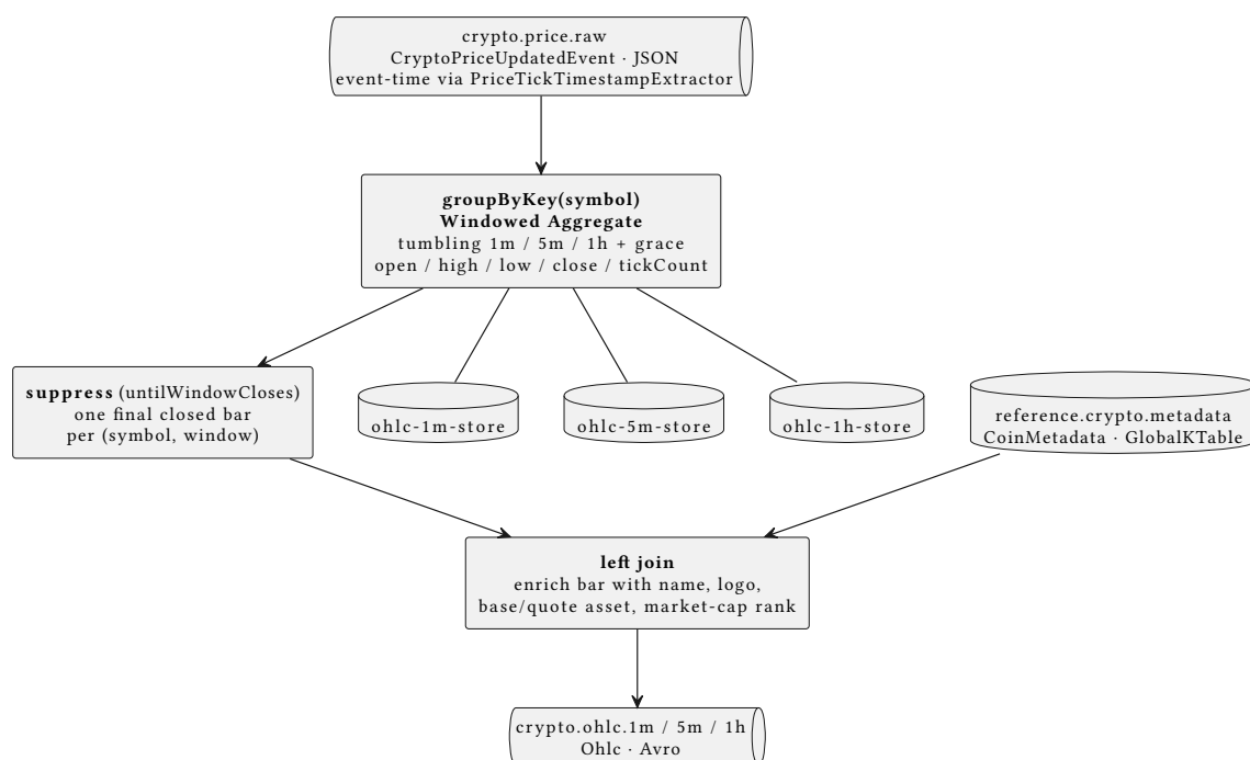
Figure 15: OHLC topology: event-time tumbling windows (1m / 5m / 1h) aggregate price ticks into closed candles, suppress(untilWindowCloses) emits one final bar per window, and a GlobalKTable left join enriches each closed bar with coin metadata before it reaches crypto.ohl.*
