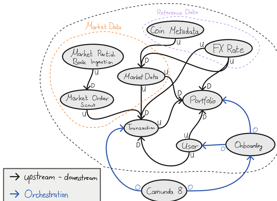
Figure 1: Context map of CryptoFlow showing bounded contexts, upstream/downstream relationships, and external systems
