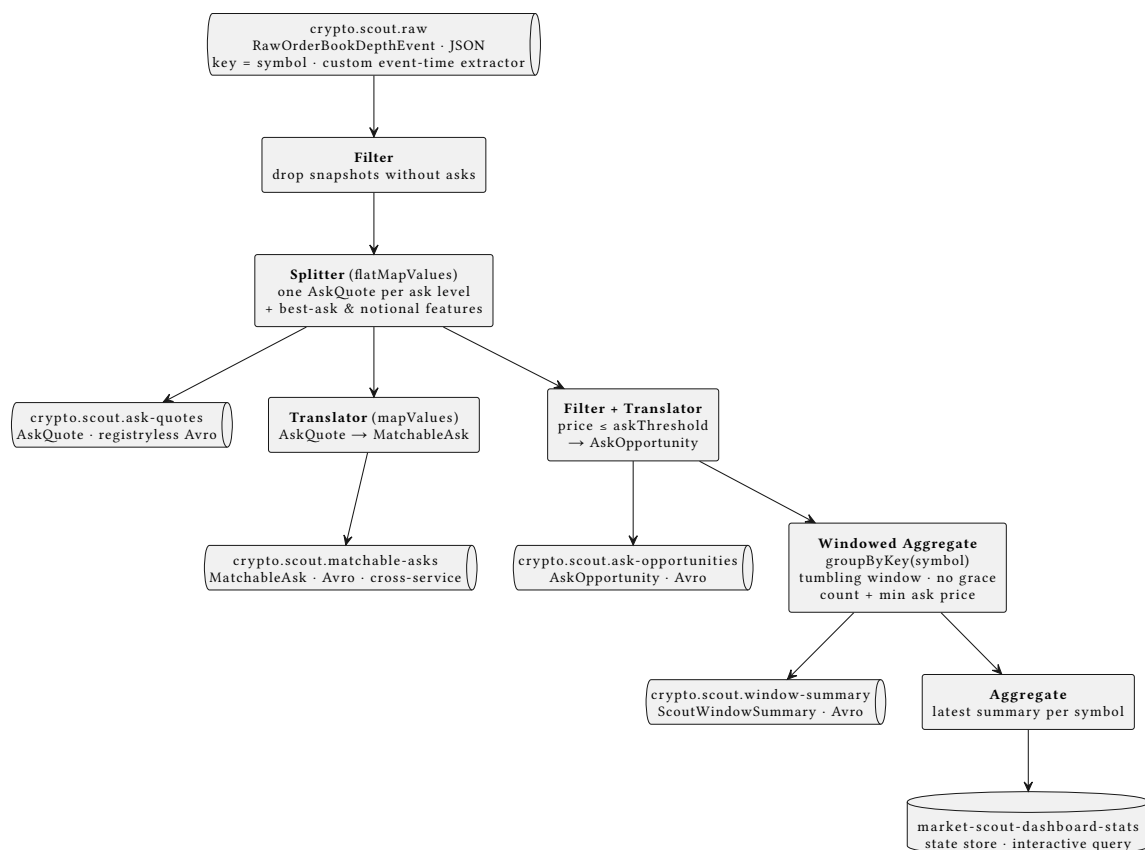
Figure 12: Market Scout Kafka Streams topology: stateless filter, splitter, and translator stages derive the ask-quote, matchable-ask, and ask-opportunity streams, which a tumbling-window aggregate folds into window summaries and a queryable dashboard-stats store
