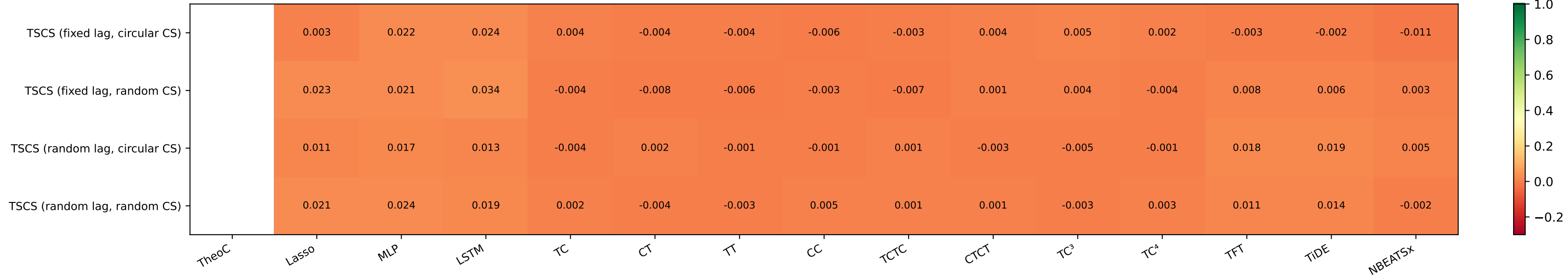
test_corr_optimal | \rho = 0.02
