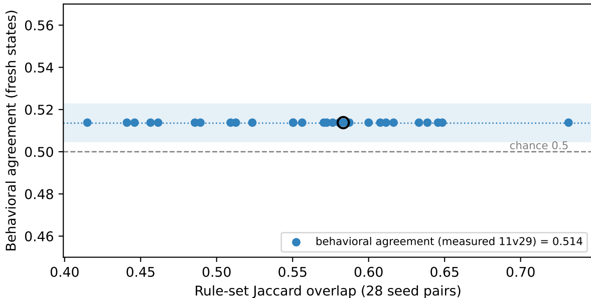
CartPole-v1: rule overlap vs behavioral agreement (overlap varies widely; agreement near chance)
