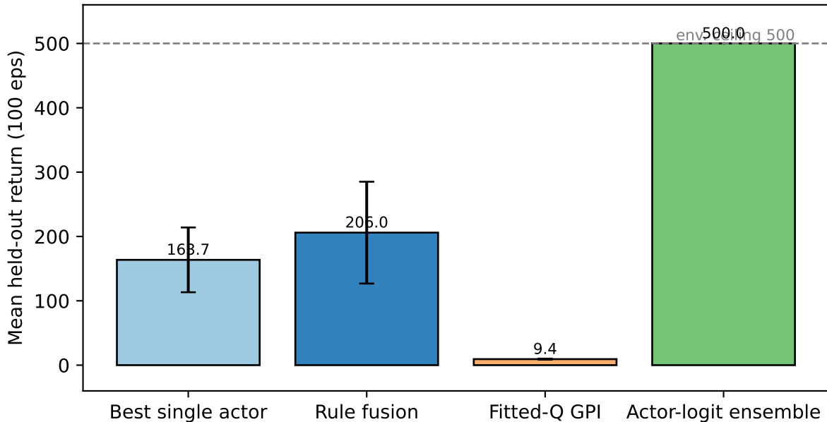
CartPole-v1: composition return by policy
